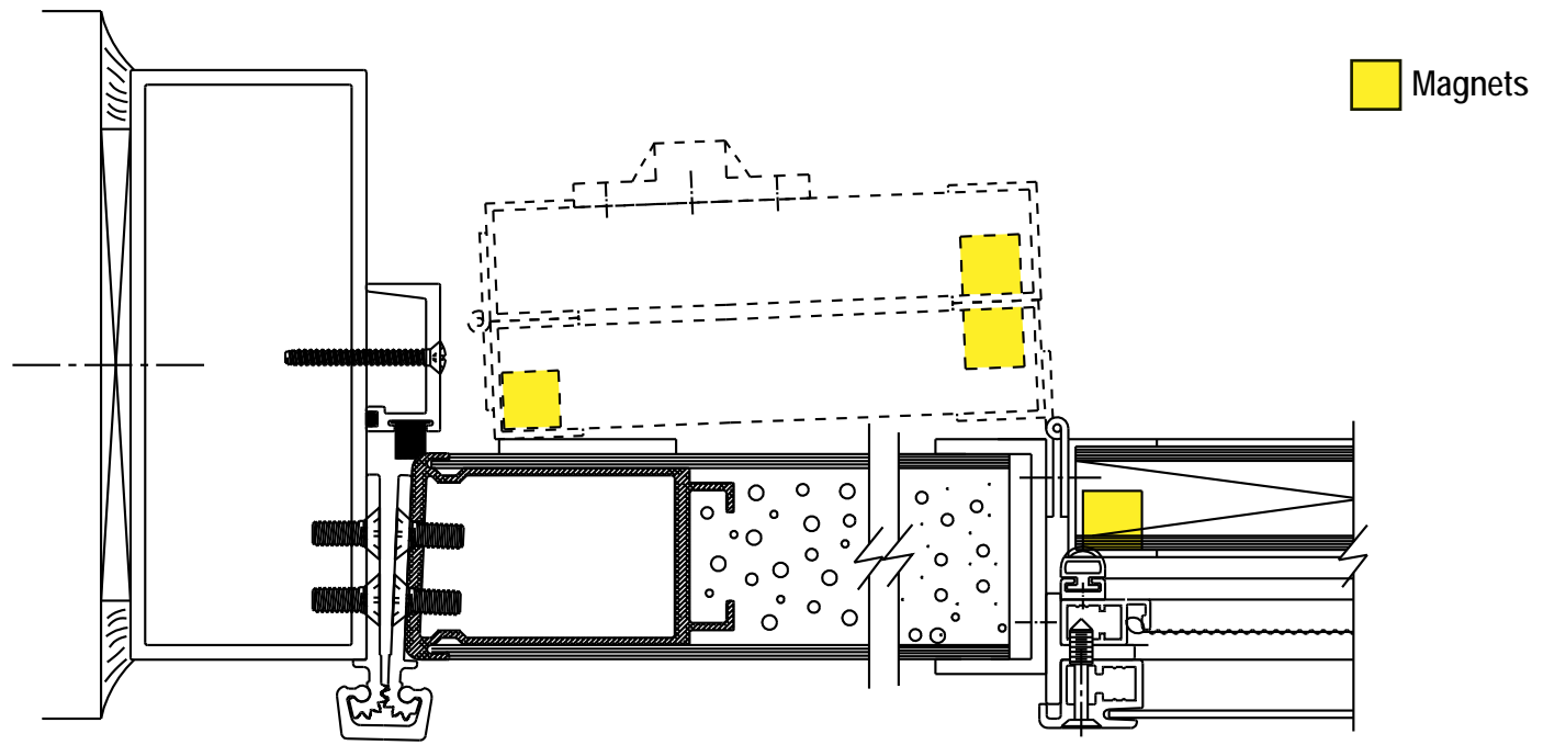
Enlarged view showing how Bi-Fold panel opens and magnetically secures to door.
