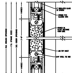
MID-PANEL DETAIL
