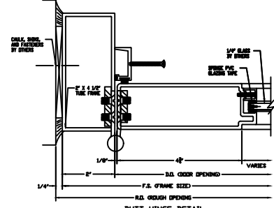
BUTT HINGE DETAIL
