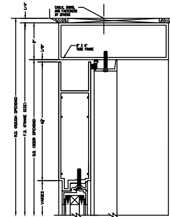
HEAD DETAIL
