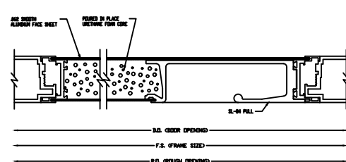
MID-PANEL DETAIL
