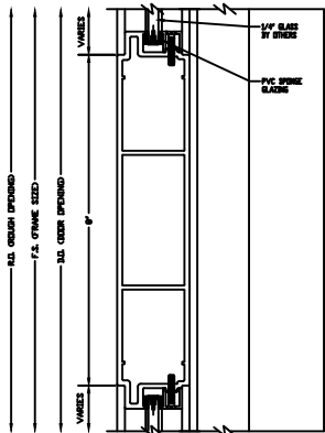
MID-RAIL DETAIL
