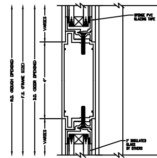
MID-RAIL DETAIL
