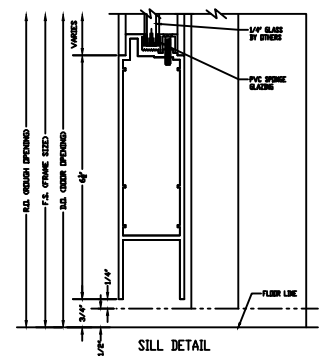
SILL DETAIL
