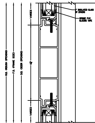
MID-RAIL DETAIL
