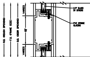
MID-RAIL DETAIL
