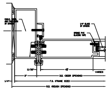
CONTINUOUS HINGE JAMB DETAIL
