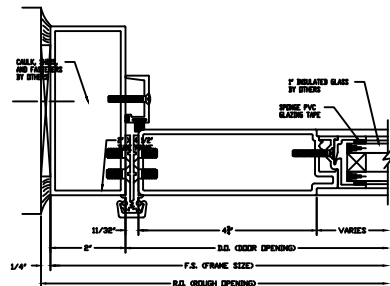
CONTINUOUS HINGE JAMB DETAIL
