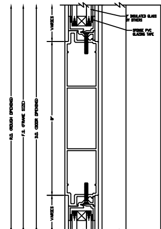
MID-RAIL DETAIL
