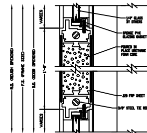
MID-PANEL DETAIL
