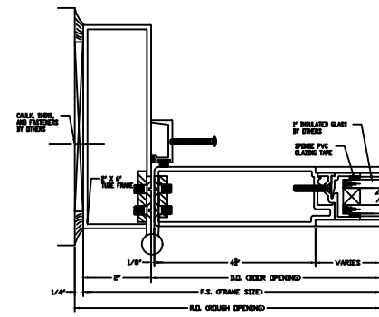
BUTT HINGE DETAIL
