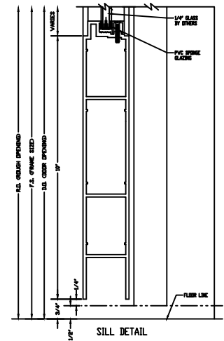
SILL DETAIL
