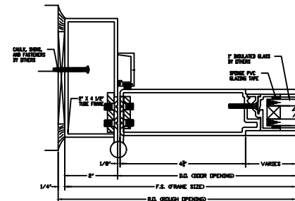
BUTT HINGE DETAIL
