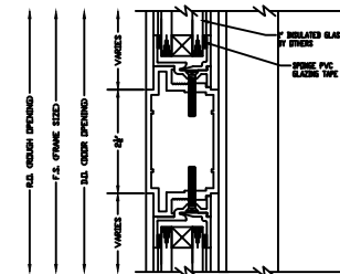
MID-RAIL DETAIL
