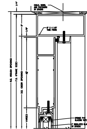
HEAD DETAIL
