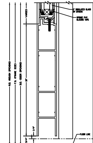
SILL DETAIL
