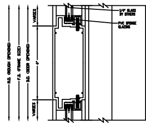
MID-RAIL DETAIL
