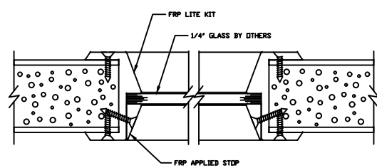
1/4" GLASS VISION LITE KIT DETAIL
