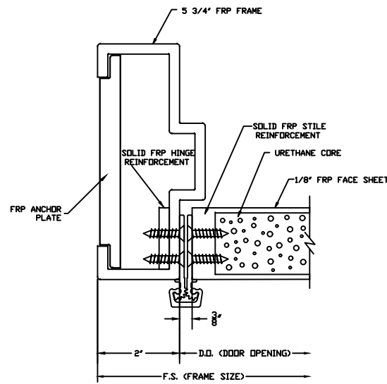
CONTINUOUS HINGE JAMB DETAIL
