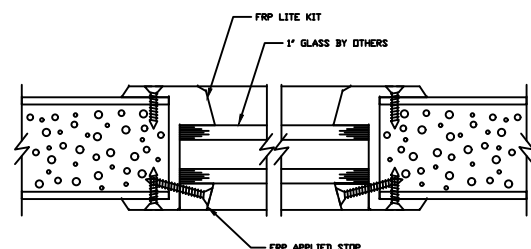
1" GLASS VISION LITE KIT DETAIL
