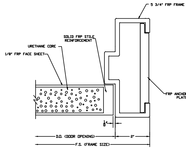
LOCK JAMB DETAIL
