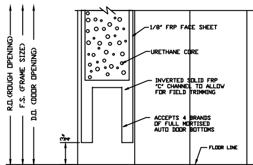
SILL DETAIL
