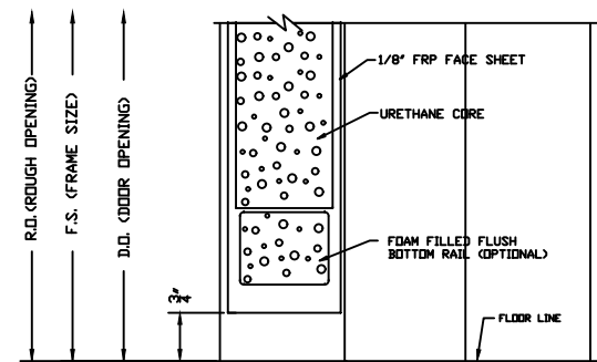
SILL DETAIL (OPTIONAL)
