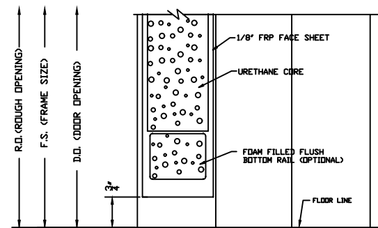
SILL DETAIL
