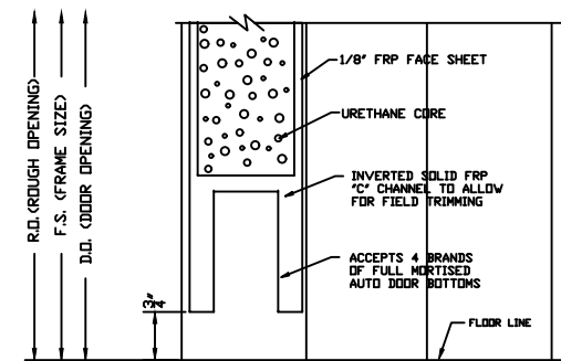
SILL DETAIL (OPTIONAL)
