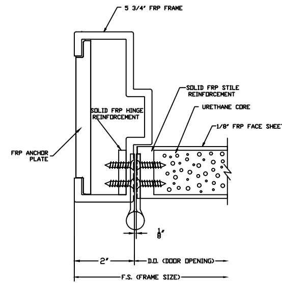
BUTT HINGE JAMB DETAIL
