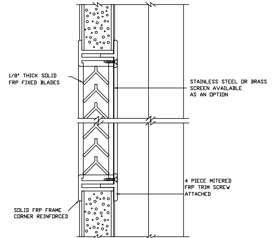
LOUVER WITH INSECT SCREEN DETAIL
