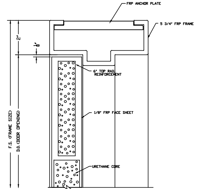
HEAD DETAIL
