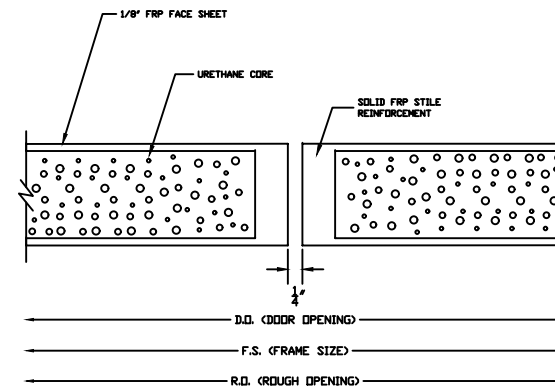
STANDARD MEETING DETAIL
