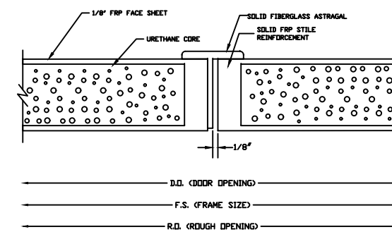
STANDARD MEETING DETAIL WITH OPTIONAL ASTRAGAL
