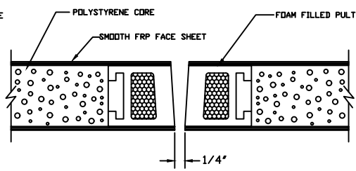
LOCK JAMB DETAIL (OPTIONAL SQUARE STILE)
