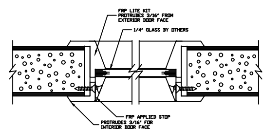
1/4" GLASS VISION LITE KIT DETAIL
