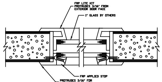
1" GLASS VISION LITE KIT DETAIL
