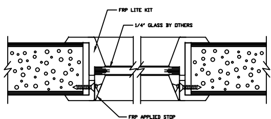
1/4" GLASS VISION LITE KIT DETAIL
