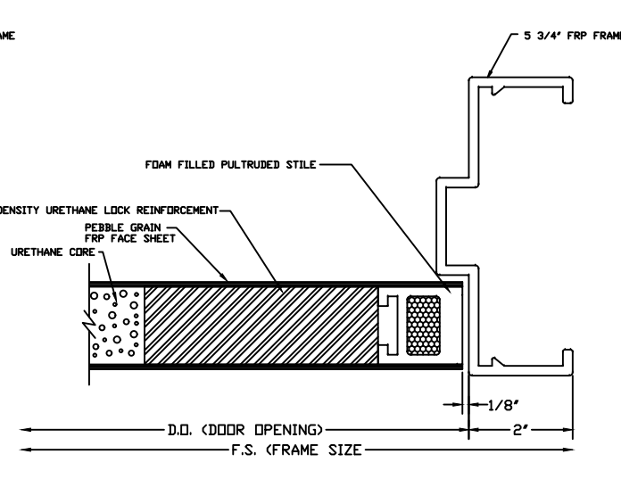
LOCK JAMB DETAIL (OPTIONAL SQUARE STILE)
