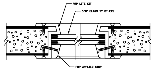
5/8" GLASS VISION LITE KIT DETAIL
