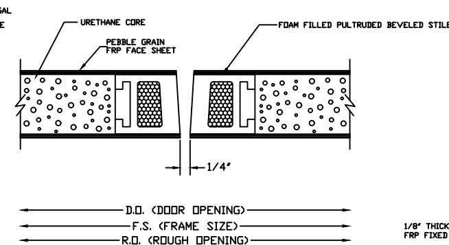
MEETING STILES WITH OPTIONAL DUAL BEVELED STILES
