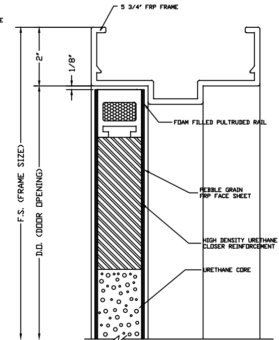
HEAD DETAIL
