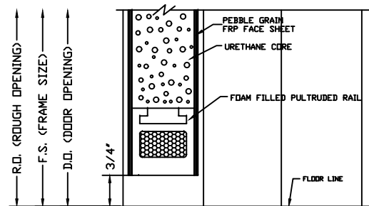
SILL DETAIL
