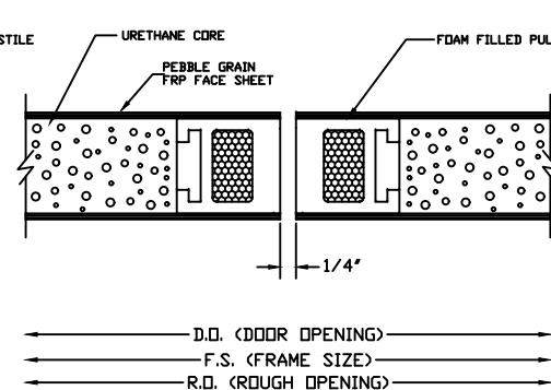
MEETING STILES OPTIONAL SQUARE STILES
