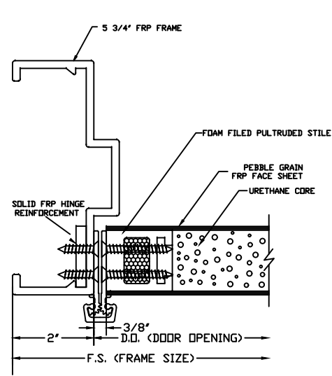
CONTINUOUS HINGE JAMB DETAIL
