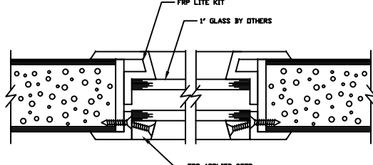
1" GLASS VISION LITE KIT DETAIL
