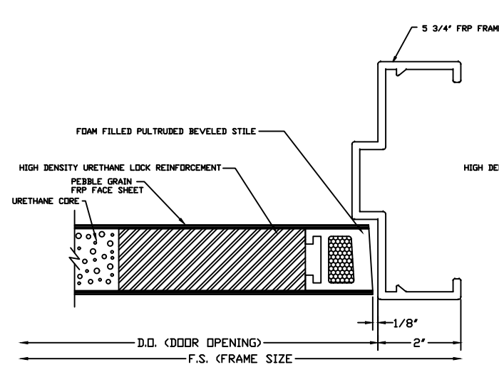
LOCK JAMB DETAIL
