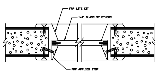
1/4" GLASS VISION LITE KIT DETAIL
