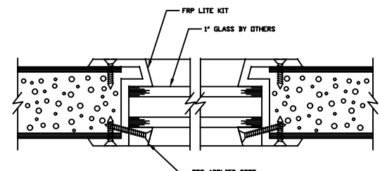
1" GLASS VISION LITE KIT DETAIL
