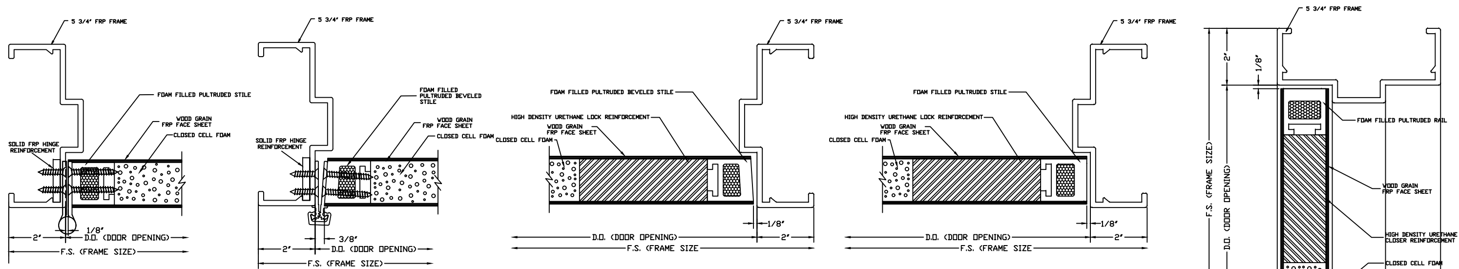
LOCK JAMB DETAIL
