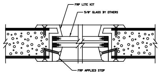
5/8" GLASS VISION LITE KIT DETAIL
