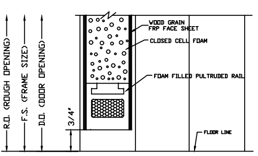
SILL DETAIL
