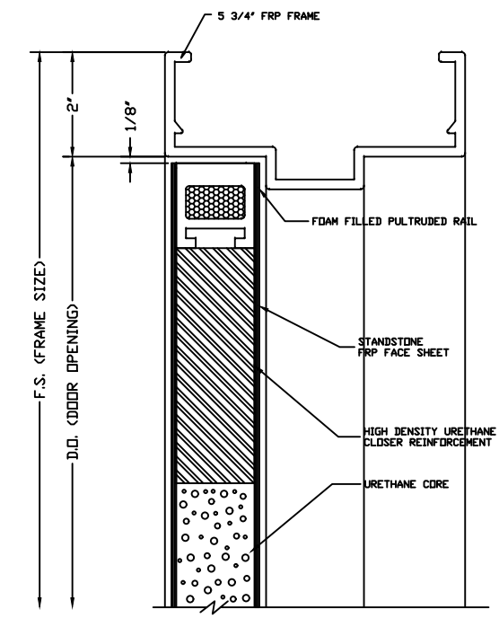
HEAD DETAIL
