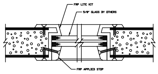
5/8" GLASS VISION LITE KIT DETAIL
