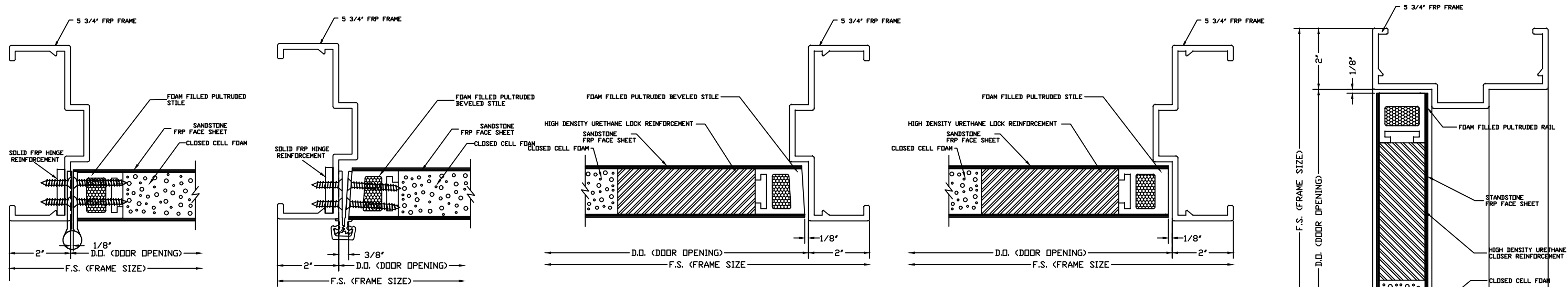
BUTT HINGE JAMB DETAIL (NOT AVAILABLE ON BEVELED STILE)
