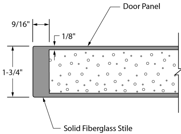
Door Stile Edges
