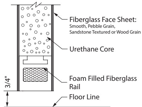
Closed Bottom Rail
