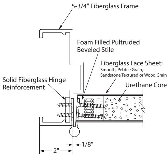
Butt Hinge with Beveled Hinge Stile
