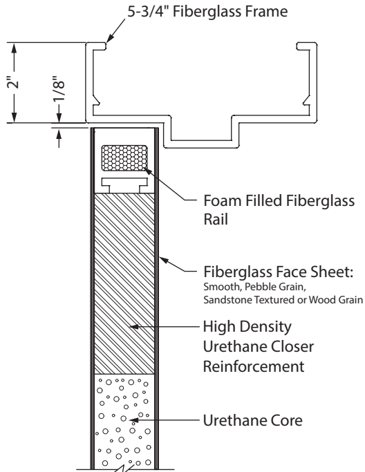
Top Rail
