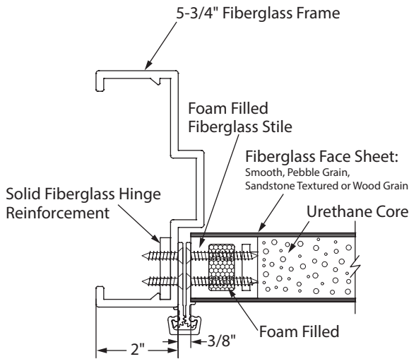
Continuous Hinge with Square Hinge Stile
