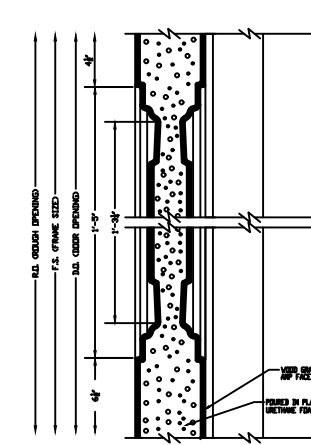
RAISED MID-PANEL DETAIL
