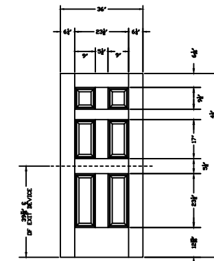
PATTERN 336A MIN= 3'- 0" x 6'- 8" MAX= 3'- 6" x 7'- 4"
