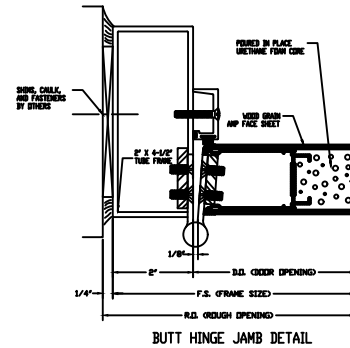
BUTT HINGE JAMB DETAIL
