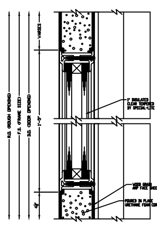
OPTIONAL TOP 1" GLAZING DETAIL
