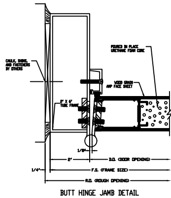
BUTT HINGE JAMB DETAIL
