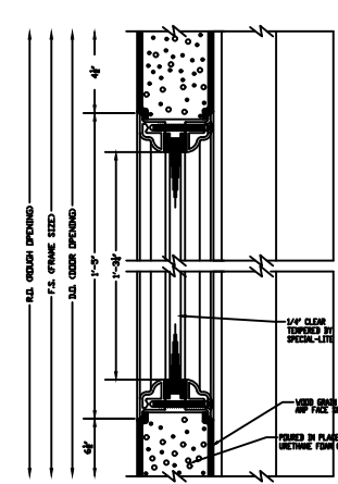
OPTIONAL MID 1/4" GLAZING DETAIL
