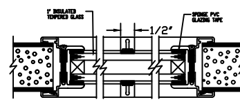
1" INS. GLASS VISION LITE KIT DETAIL WITH EXTERNAL MUNTIN
