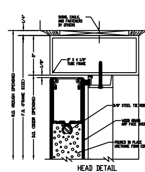
HEAD DETAIL
