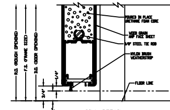
SILL DETAIL
