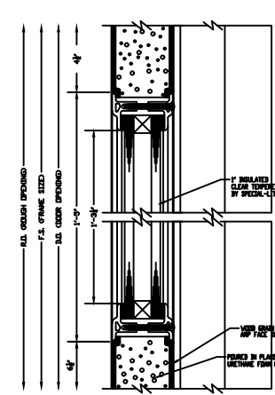
OPTIONAL MID 1" GLAZING DETAIL
