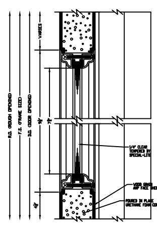
OPTIONAL TOP 1/4" GLAZING DETAIL
