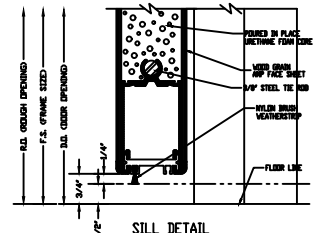
SILL DETAIL
