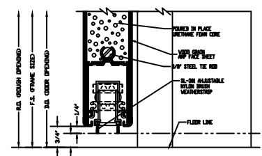
SILL DETAIL (OPTIONAL)
