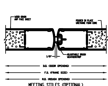
MEETING STILES (OPTIONAL)
