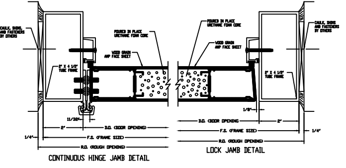
CONTINUOUS HINGE JAMB DETAIL
