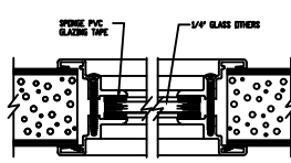
1/4" GLASS VISION LITE KIT DETAIL
