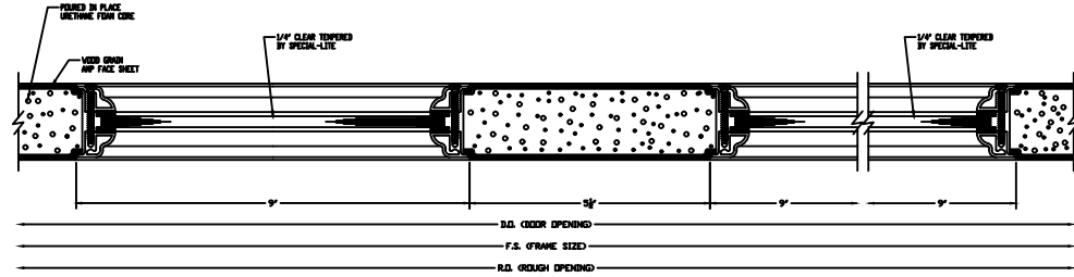
OPTIONAL 1/4" GLAZING HORIZONTAL DETAIL
