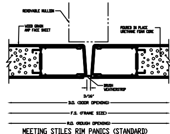
MEETING STILES RIM PANICS (STANDARD)
