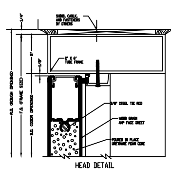
HEAD DETAIL
