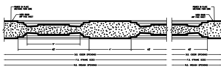
RAISED PANEL HORIZONTAL DETAIL
