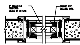
1" INS. GLASS VISION LITE KIT DETAIL
