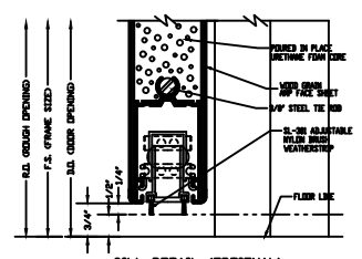
SILL DETAIL (OPTIONAL)
