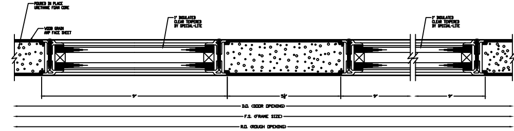
OPTIONAL 1" GLAZING HORIZONTAL DETAIL
