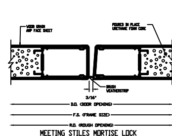
MEETING STILES MORTISE LOCK
