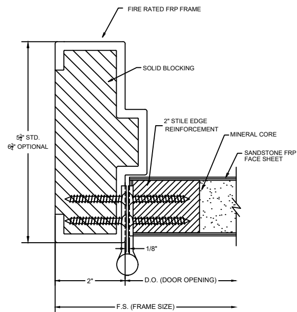
BUTT HINGE DETAIL
