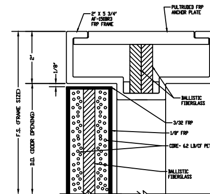
HEAD DETAIL
