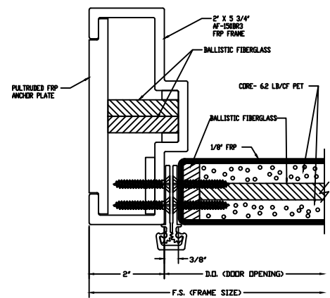
CONTINUOUS HINGE JAMB DETAIL
