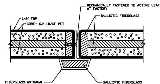
MEETING STILES WITH ASTRAGAL
