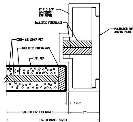
LOCK JAMB DETAIL
