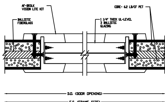
VISION-LITE DETAIL
