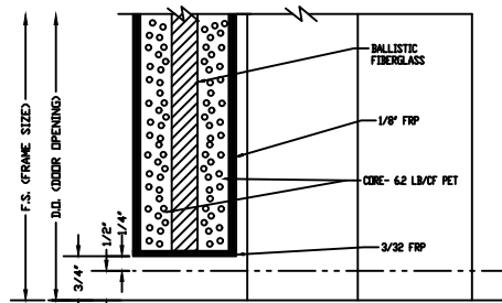
SILL DETAIL
