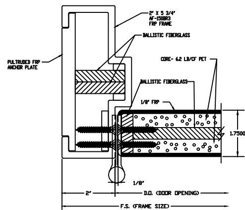
BUTT HINGE JAMB DETAIL
