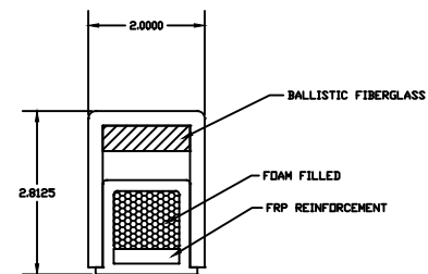
BALLISTIC MULLION DETAIL
