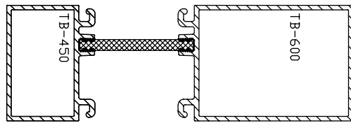
SL-600TB 2" x 6" x 0.080" Double Pocket Tube Mullion
