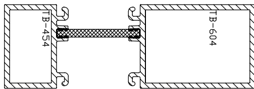
SL-600TB 2" x 6" x 0.125" Double Pocket Tube Mullion
