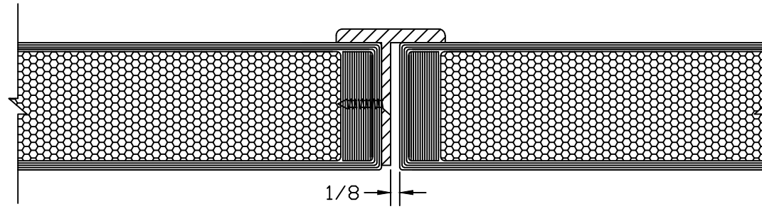
FRP Astragal At Meeting Pair
