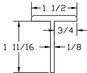
STANDARD T ASTRAGAL
