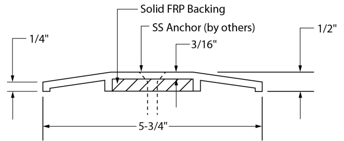
Standard Saddle Threshold
