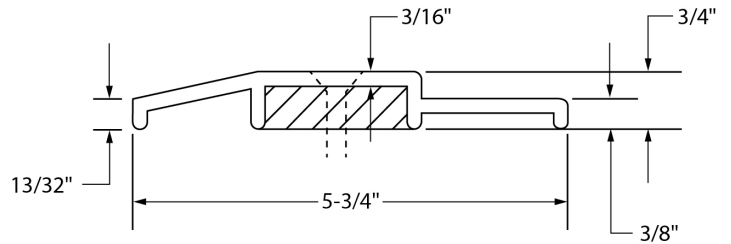
Standard Bumper Threshold
