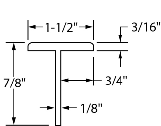
Standard T Astragal
