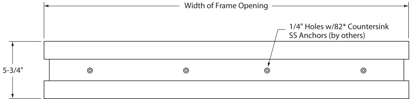
Standard Threshold Anchorage
