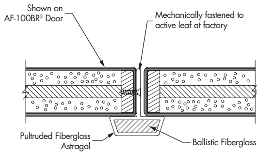
Ballistic T-Astragal
