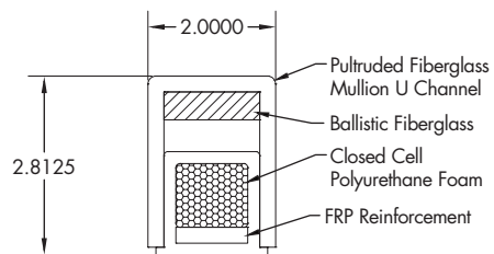
Ballistic Mullion
