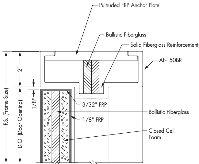
Head Detail
