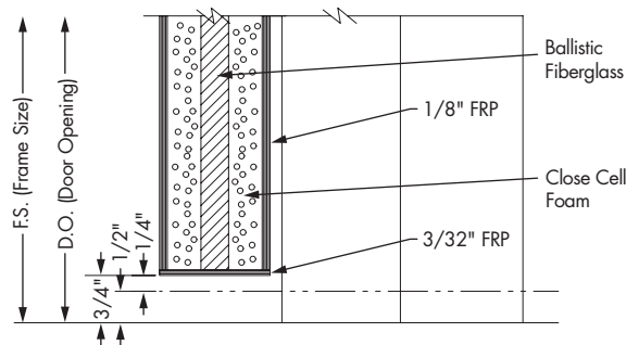
Sill Detail
