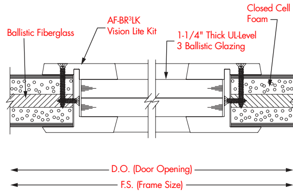
Vision Lite
