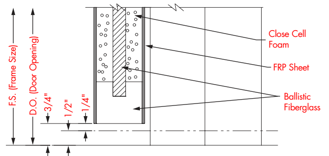
Sill Detail
