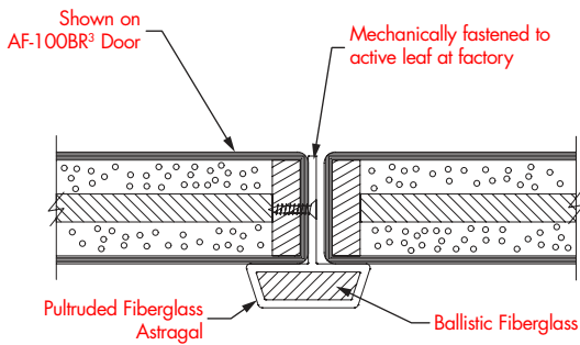
Ballistic T-Astragal
