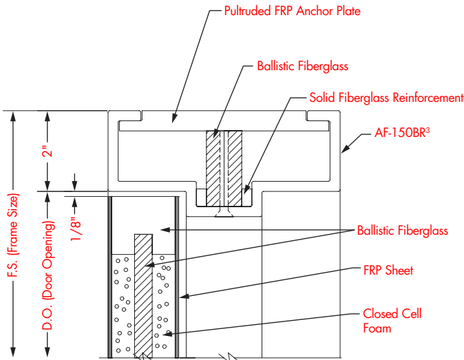
Head Detail
