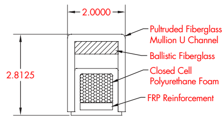
Ballistic Mullion
