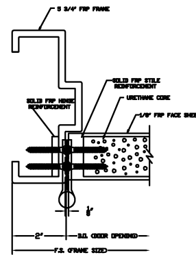
BUTT HINGE JAMB DETAIL
