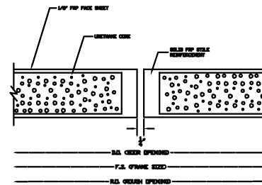
STANDARD MEETING DETAIL
