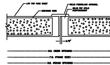
STANDARD MEETING DETAIL WITH OPTIONAL ASTRAGAL
