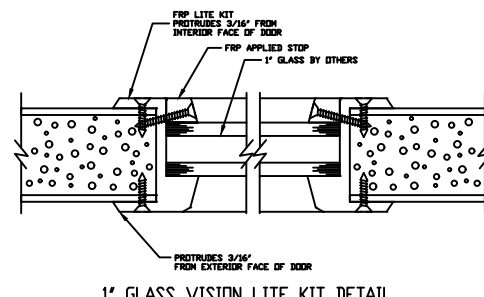
1" GLASS VISION LITE KIT DETAIL
