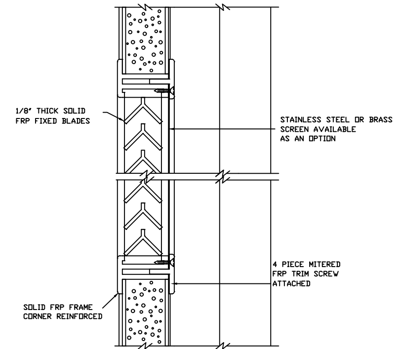
LOUVER WITH INSECT SCREEN DETAIL
