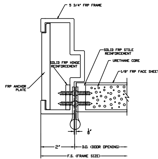
BUTT HINGE JAMB DETAIL
