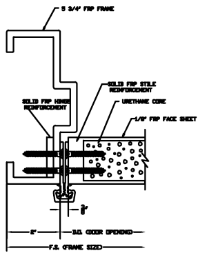
CONTINUOUS HINGE JAMB DETAIL
