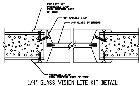
1/4" GLASS VISION LITE KIT DETAIL
