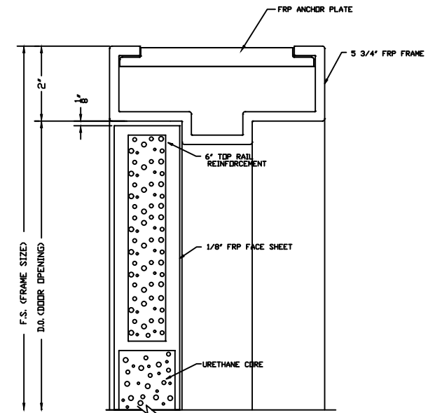
HEAD DETAIL
