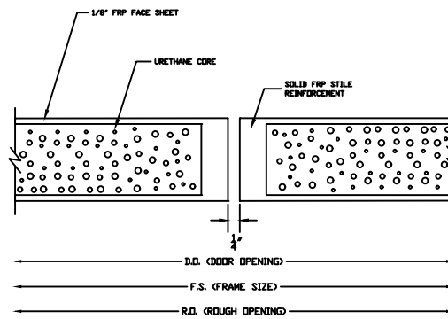
STANDARD MEETING DETAIL
