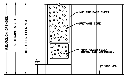
SILL DETAIL (OPTIONAL)
