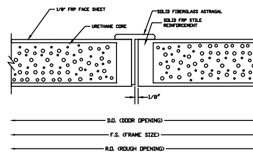
STANDARD MEETING DETAIL WITH OPTIONAL ASTRAGAL
