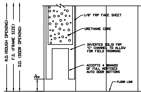
SILL DETAIL
