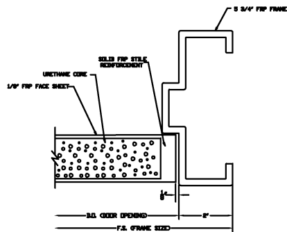
LOCK JAMB DETAIL
