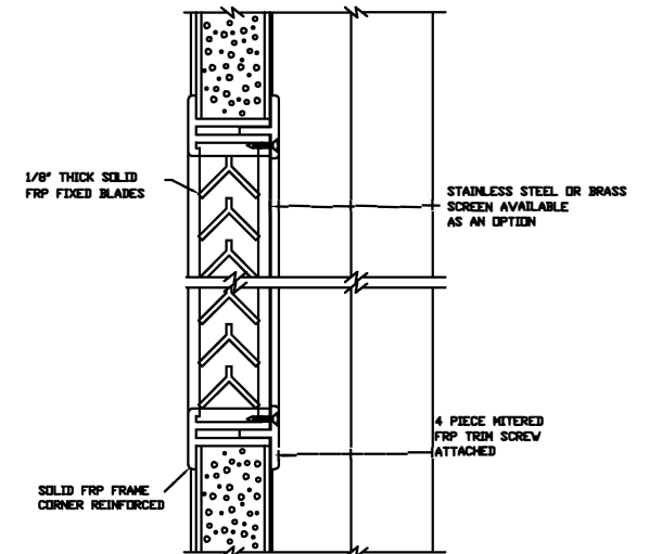
LOUVER WITH INSECT SCREEN DETAIL
