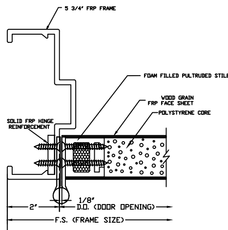
BUTT HINGE JAMB DETAIL (NOT AVAILABLE ON BEVELED STILE)
