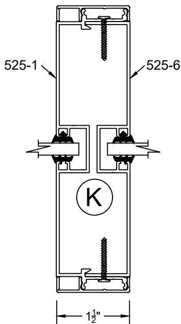
1 1/2" VERTICAL MULLION
