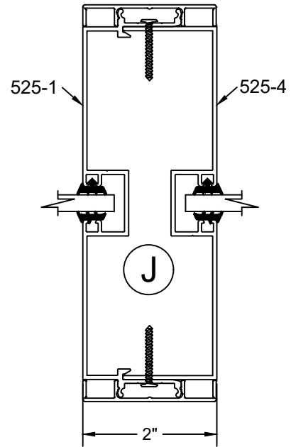
2" VERTICAL MULLION
