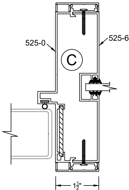
DOOR JAMB WITH SIDELITE 1 1/2" MULLION
