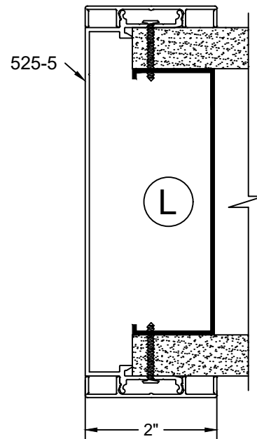
CASED OPENING JAMB
