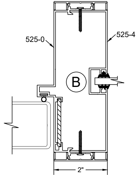
DOOR JAMB WITH SIDELITE 2" MULLION
