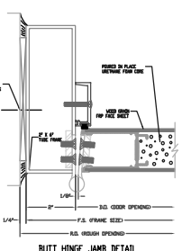
BUTT HINGE JAMB DETAIL
