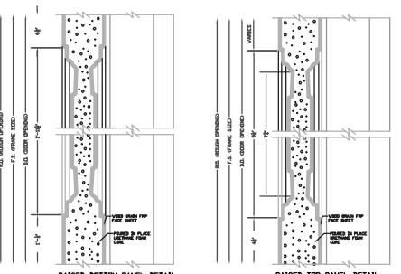
RAISED BOTTOM PANEL DETAIL
