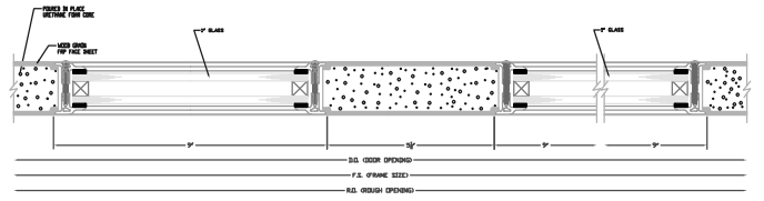
OPTIONAL 1" GLAZING HORIZONTAL DETAIL
