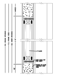
OPTIONAL TOP 1" GLAZING DETAIL
