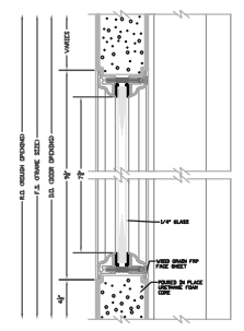
OPTIONAL TOP 1/4" GLAZING DETAIL
