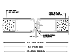
MEETING STILES (OPTIONAL)
