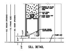
SILL DETAIL
