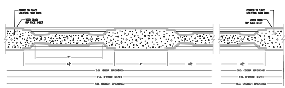
RAISED PANEL HORIZONTAL DETAIL
