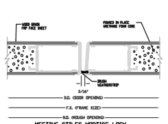
MEETING STILES MORTISE LOCK
