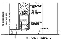
SILL DETAIL (OPTIONAL)
