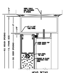
HEAD DETAIL
