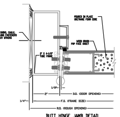
BUTT HINGE JAMB DETAIL
