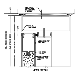
HEAD DETAIL
