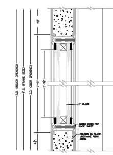
OPTIONAL MID 1" GLAZING DETAIL
