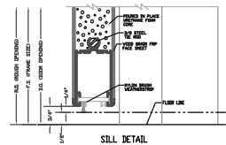
SILL DETAIL
