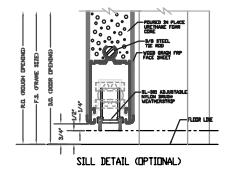
SILL DETAIL (OPTIONAL)
