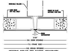
MEETING STILES RM PANICS (STANDARD)
