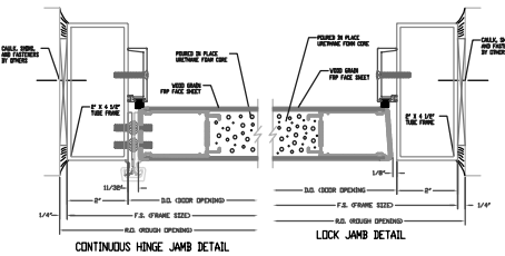
CONTINUOUS HINGE JAMB DETAIL
