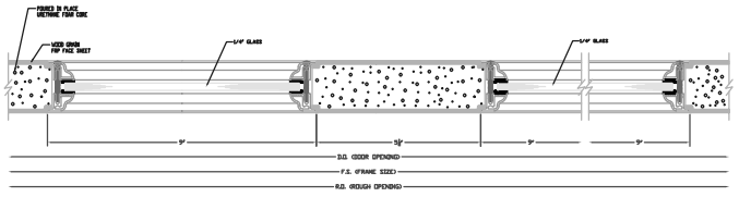
OPTIONAL 1/4" GLAZING HORIZONTAL DETAIL
