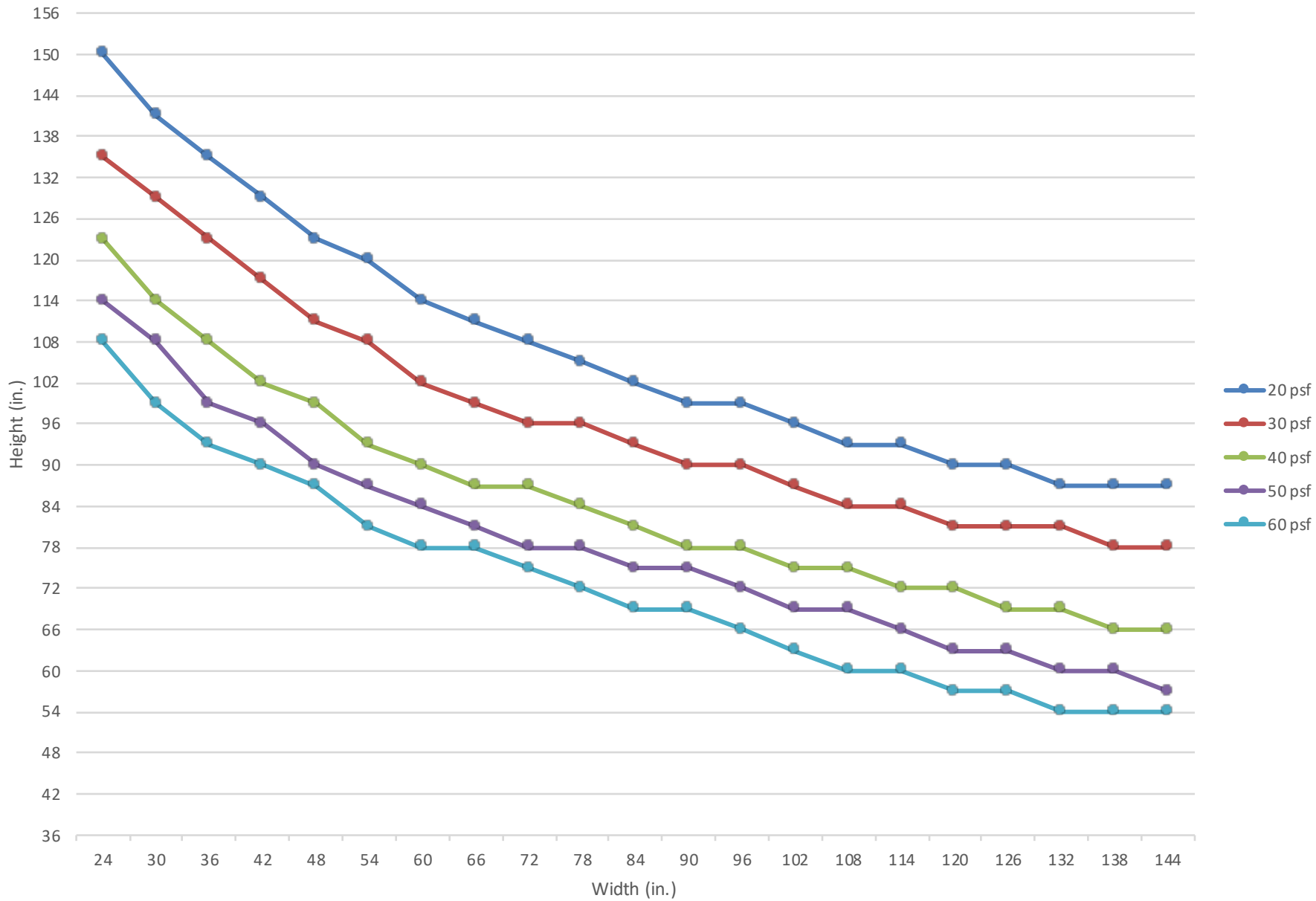
SL-240, 2" x 4" Heavy Duty Framing with Applied Stop
