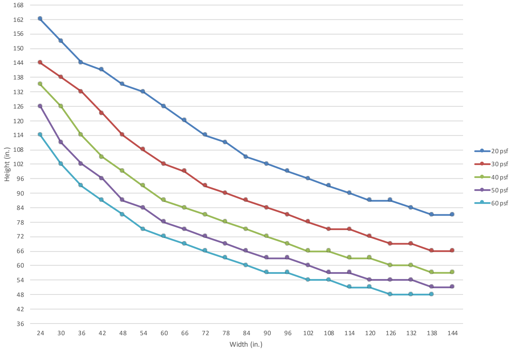
SL-245, 2" x 4-1/2" Heavy Duty Framing with Applied Stops
