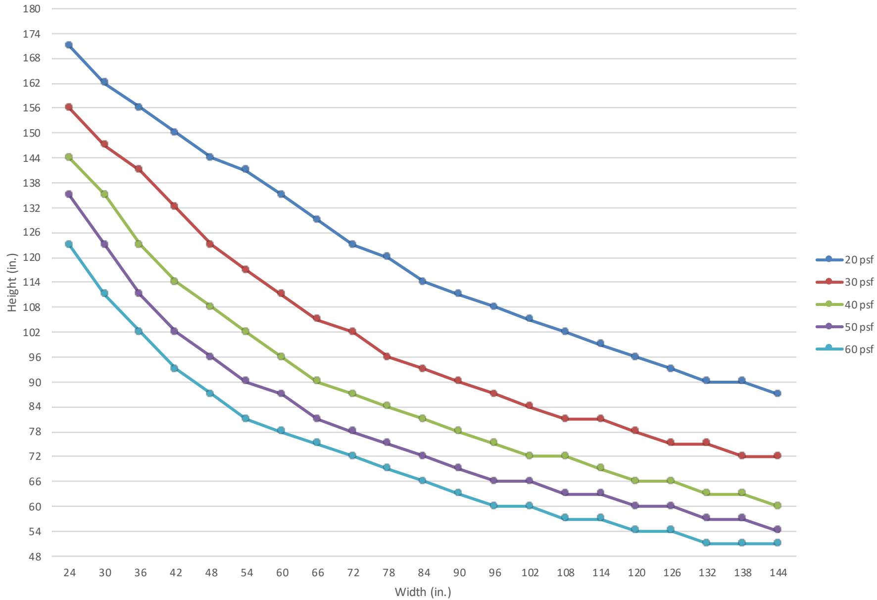
SL-250, 2" x 5" Heavy Duty Framing with Applied Stop
