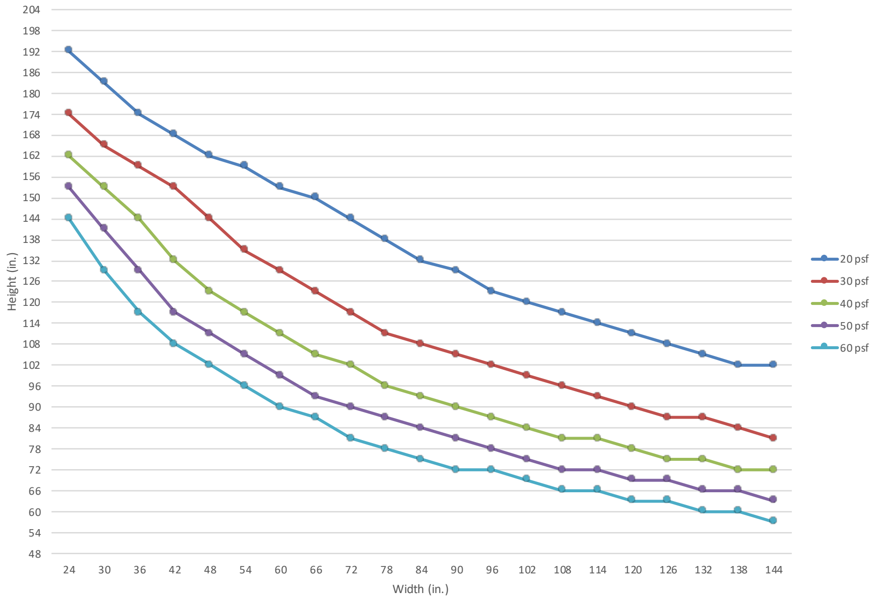
SL-260, 2" x 6" Heavy Duty Framing with Applied Stop
