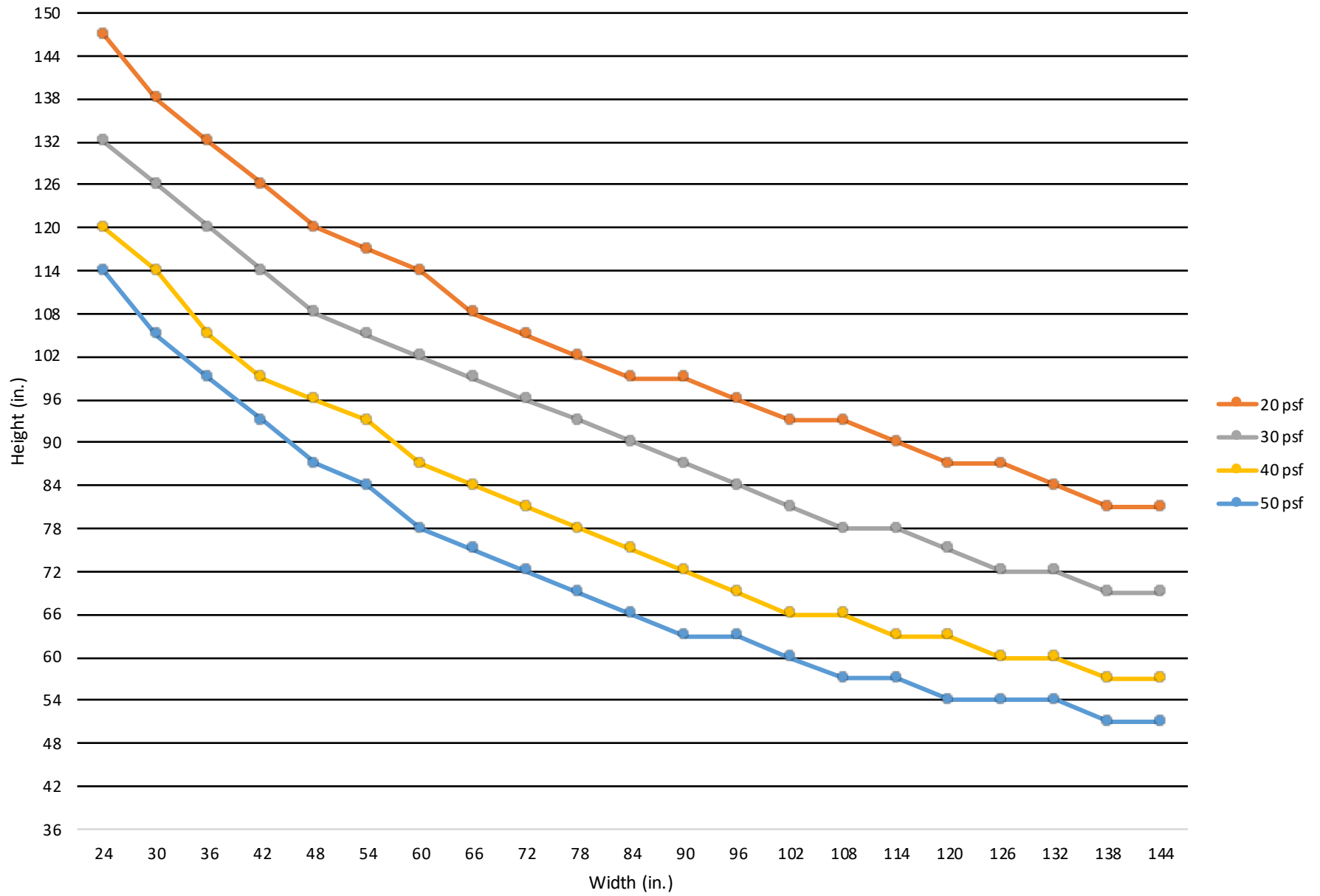
SL-450TB, 2" x 4.5" x 0.125" Thermally Broken Framing
