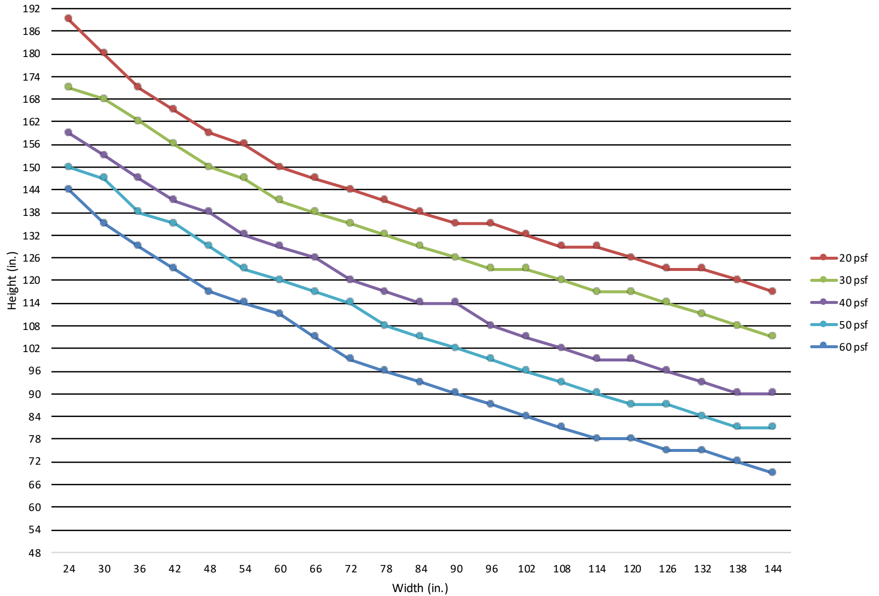
SL-55, 1-3/4" x 6" Heavy Duty Framing with Applied Stops
