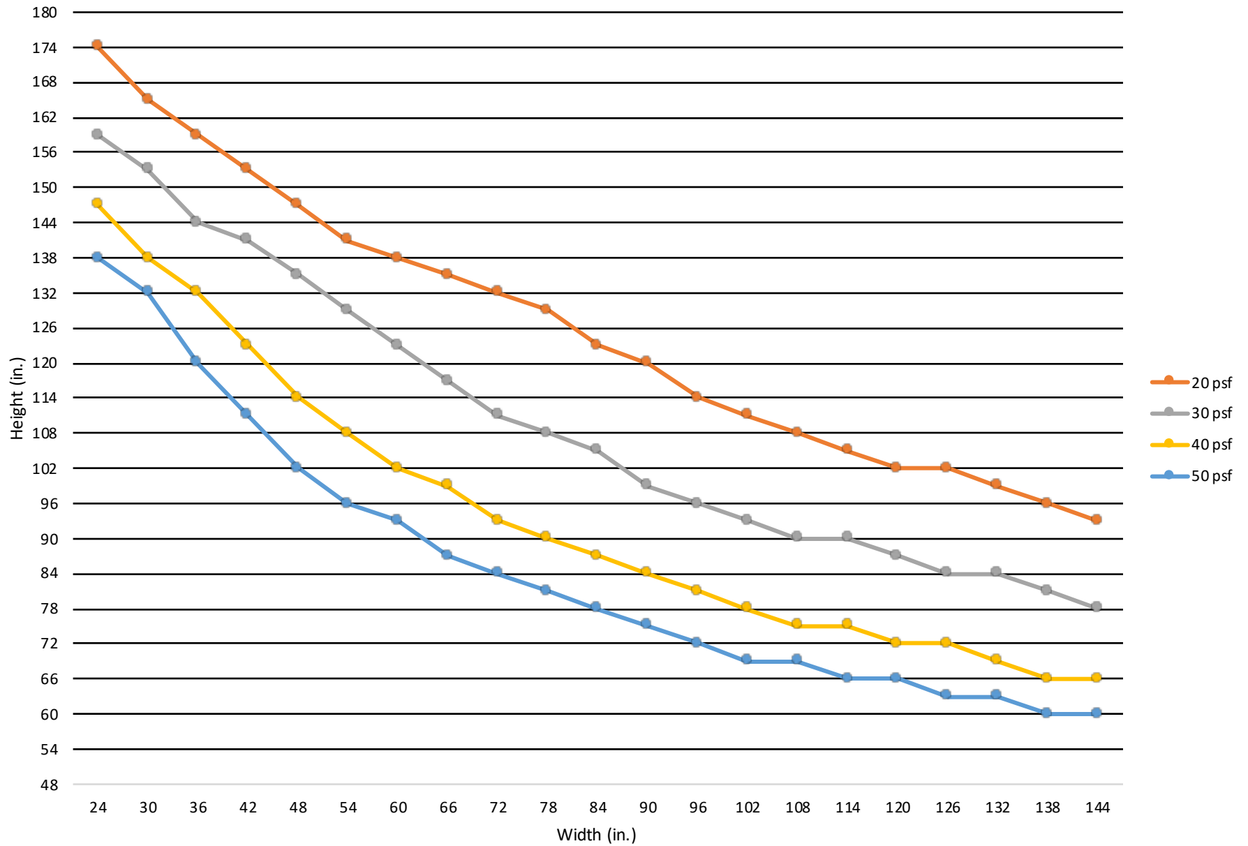
SL-600TB, 2" x 6" x 0.125" Thermally Broken Framing
