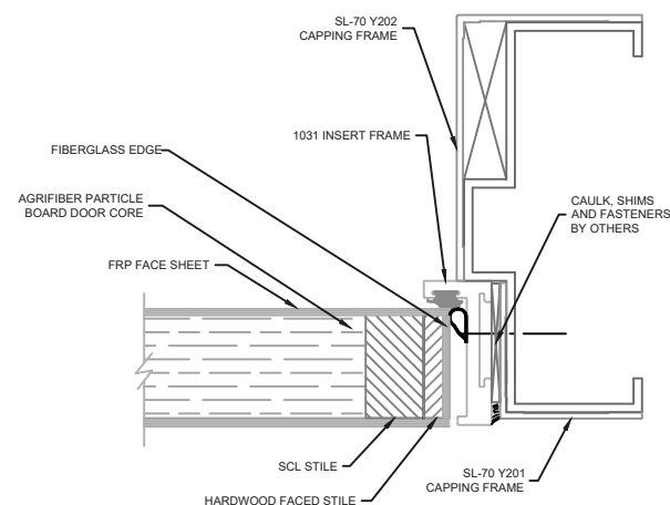
LOCK JAMB DETAIL WITH CAPPING
