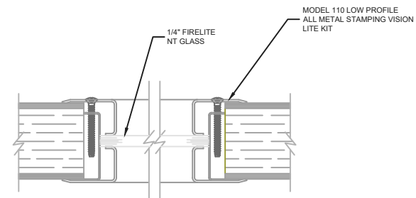
VISION LITE KIT DETAIL 1/4" GLASS
