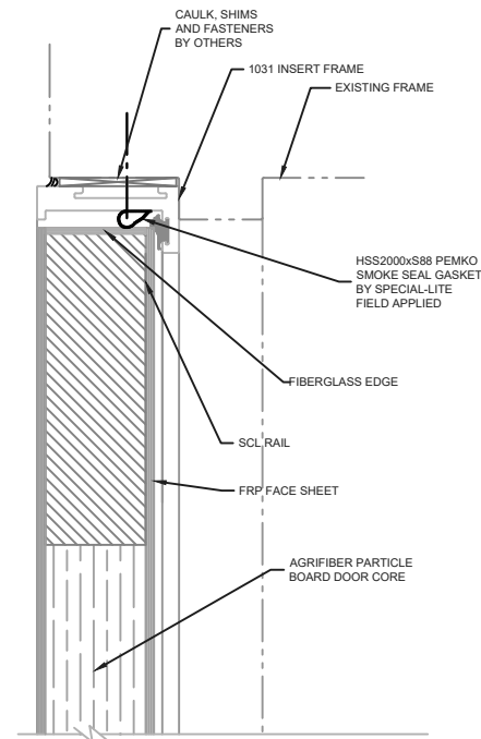
HEAD DETAIL
