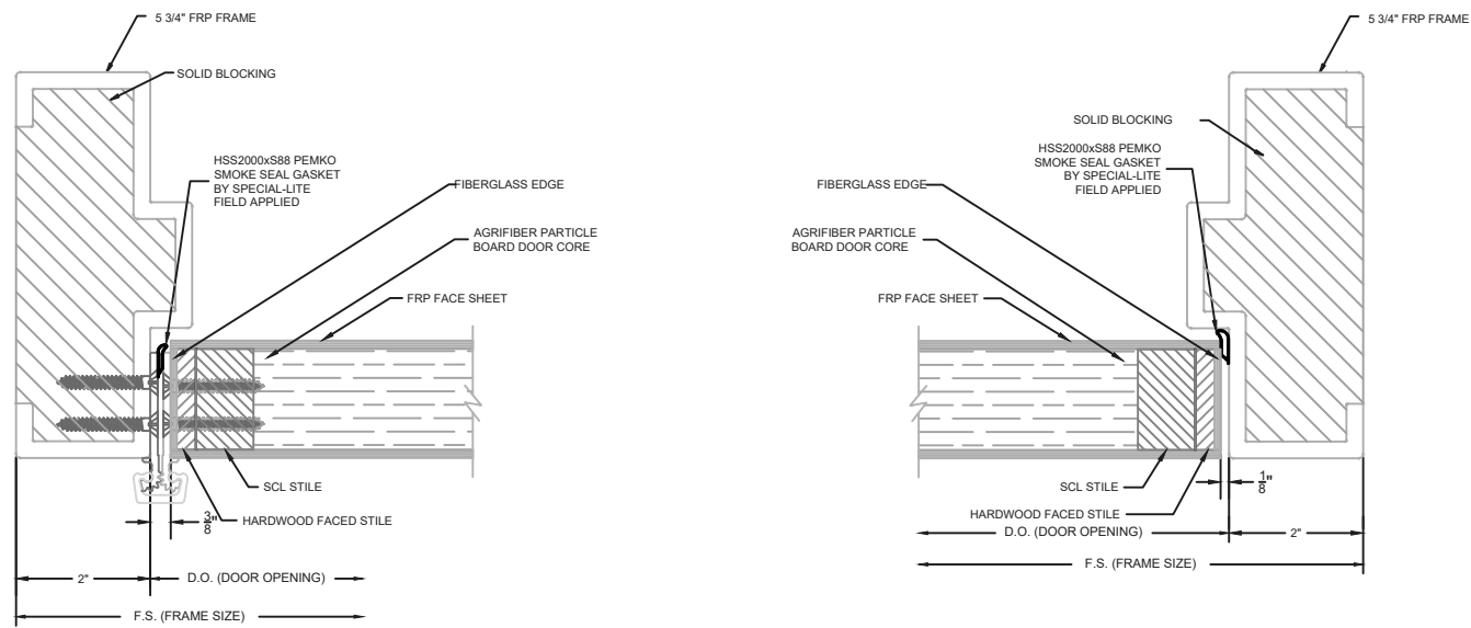
CONTINUOUS HINGE JAMB DETAIL
