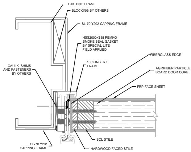
CONTINUOUS HINGE JAMB DETAIL
