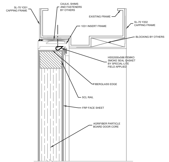
HEAD DETAIL WITH CAPPING
