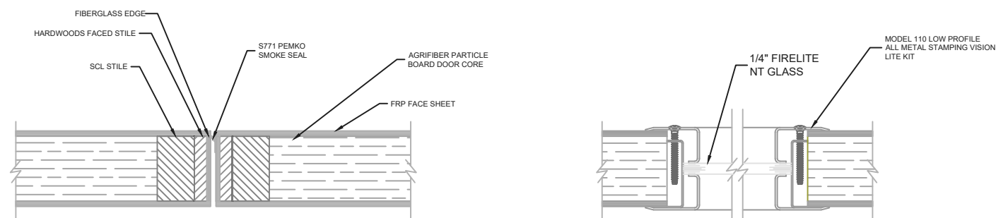
LOCKSET MEETING DETAIL
