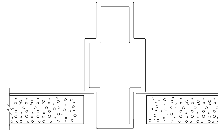
6-3/4" AF CENTER POST (FIXED OR REMOVABLE)
