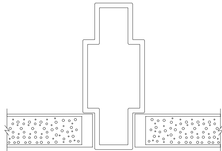
7-3/4" AF CENTER POST (FIXED OR REMOVABLE)
