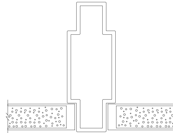
8-3/4" AF CENTER POST (FIXED OR REMOVABLE)
