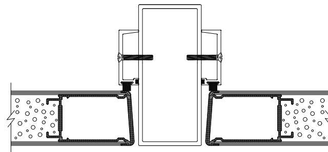
2" x 4-1/2" FRAMING FIXED MULLION OR SL-61 REMOVABLE POST
