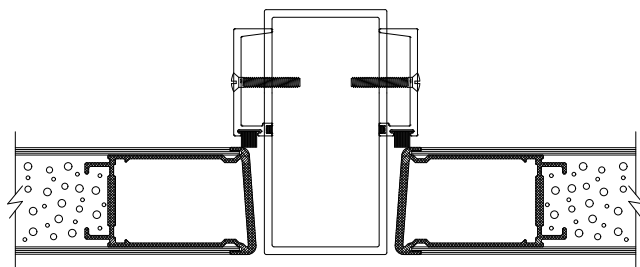
2" x 4" FRAMING FIXED MULLION OR SL-61 REMOVABLE POST
