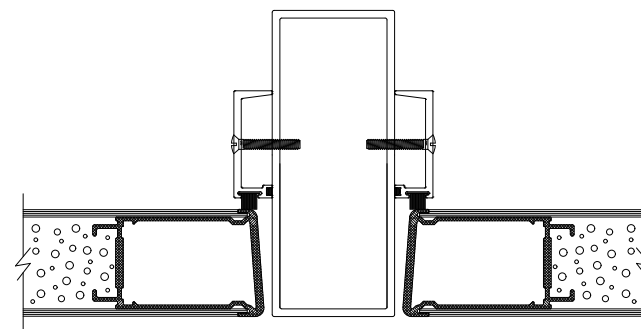
2" x 5" FRAMING FIXED MULLION OR SL-61 REMOVABLE POST
