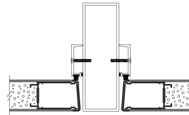
2" x 6" FRAMING FIXED MULLION OR SL-61 REMOVABLE POST
