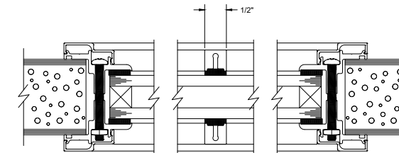
1" GLASS SECURELITE KIT DETAIL, 1/2" BITE WITH 1/2" EXTERNAL MUNTIN
