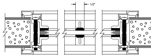
1/4" GLASS SECURELITE KIT DETAIL, 1/2" BITE WITH 1/2" EXTERNAL MUNTIN
