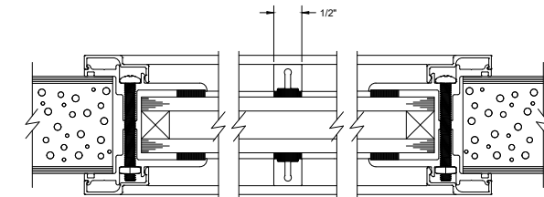
1" GLASS SECURELITE KIT DETAIL, 1" BITE WITH 1/2" EXTERNAL MUNTIN
