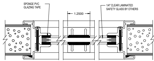
1/4" GLASS VISION LITE KIT DETAIL WITH 1-1/4" EXTERNAL MUNTIN
