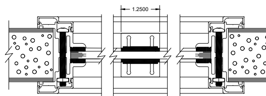
1/4" GLASS SECURELITE KIT DETAIL, 1/2" BITE WITH 1-1/4" EXTERNAL MUNTIN
