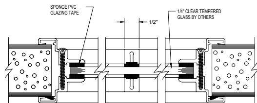
1/4" GLASS VISION LITE KIT DETAIL WITH 1/2" EXTERNAL MUNTIN
