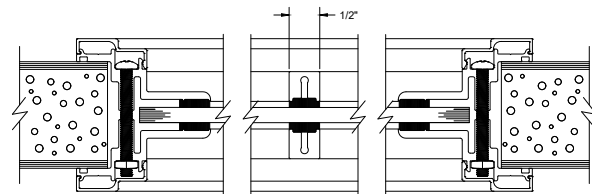
1/4" GLASS SECURELITE KIT DETAIL, 1" BITE WITH 1/2" EXTERNAL MUNTIN
