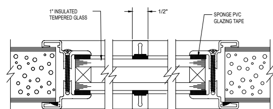
1" INS. GLASS VISION LITE KIT DETAIL WITH 1/2" EXTERNAL MUNTIN
