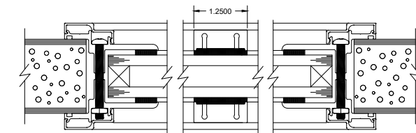
1" GLASS SECURELITE KIT DETAIL, 1" BITE WITH 1-1/4" EXTERNAL MUNTIN
