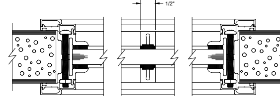
1/2" GLASS SECURELITE KIT DETAIL, 1/2" BITE WITH 1/2" EXTERNAL MUNTIN
