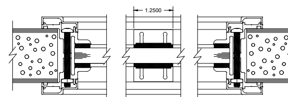
1/2" GLASS SECURELITE KIT DETAIL, 1/2" BITE WITH 1-1/4" EXTERNAL MUNTIN
