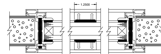
1" GLASS SECURELITE KIT DETAIL, 1/2" BITE WITH 1-1/4" EXTERNAL MUNTIN
