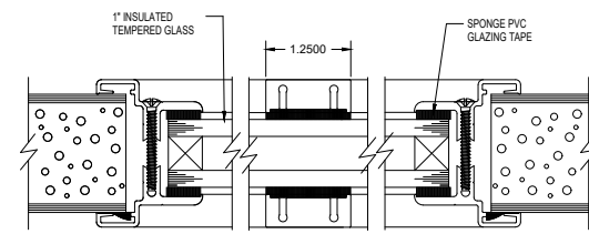
1" INS. GLASS VISION LITE KIT DETAIL WITH 1-1/4" EXTERNAL MUNTIN
