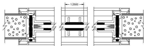
1/4" GLASS SECURELITE KIT DETAIL, 1" BITE WITH 1-1/4" EXTERNAL MUNTIN
