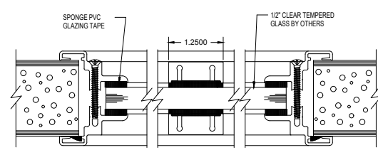
1/2" GLASS VISION LITE KIT DETAIL WITH 1-1/4" EXTERNAL MUNTIN
