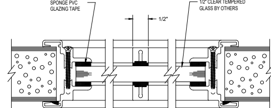
1/2" GLASS VISION LITE KIT DETAIL WITH 1/2" EXTERNAL MUNTIN
