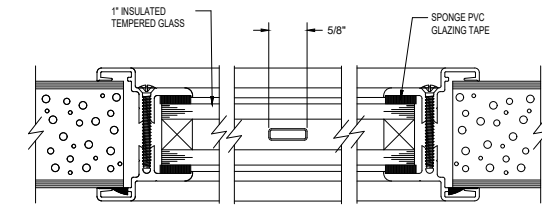
1" INS. GLASS VISION LITE KIT DETAIL WITH INTERNAL MUNTIN
