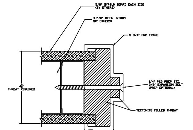
PUNCH AND DIMPLE TUCK FRP FRAME @ METAL STUDS
