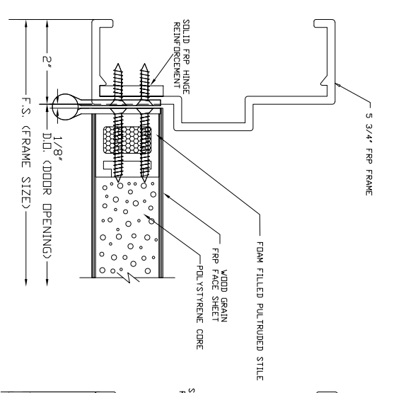
1 BUTT HINGE JAMB DETAIL (NOT AVAILABLE ON BEVELED STILES) 1:1
