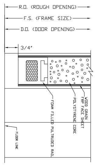
10 SILL DETAIL (FLUSH BOTTOM) 1:1
