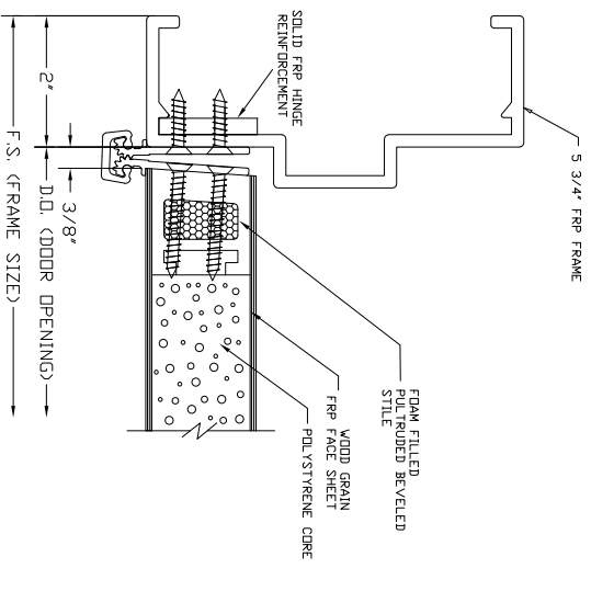
2 CONTINUOUS HINGE JAMB DETAIL 1:1
