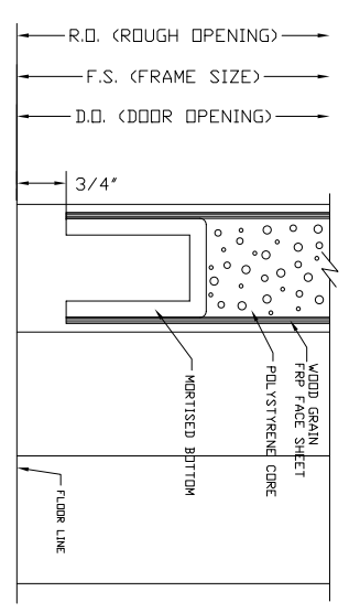
11 SILL DETAIL (MORTISED BOTTOM) 1:1
