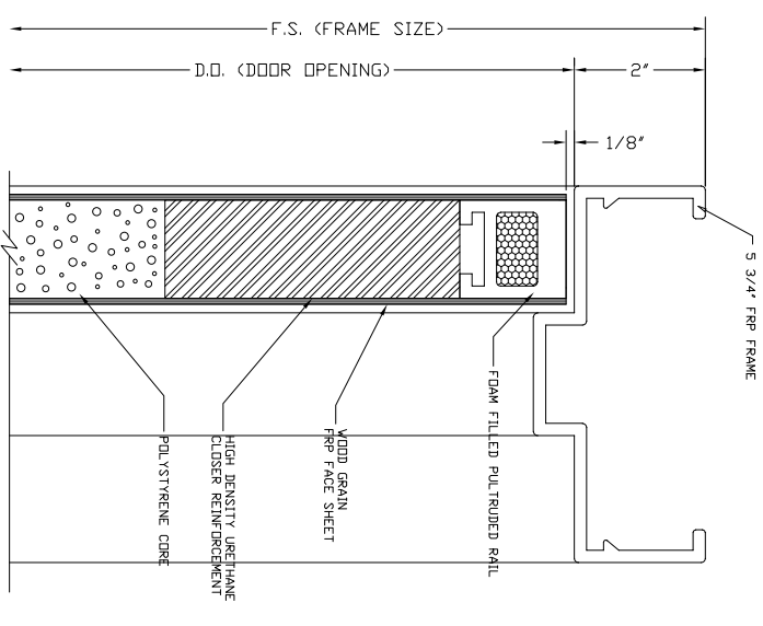
5 HEAD DETAIL 1:1
