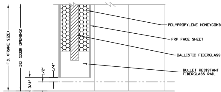
SILL DETAIL
