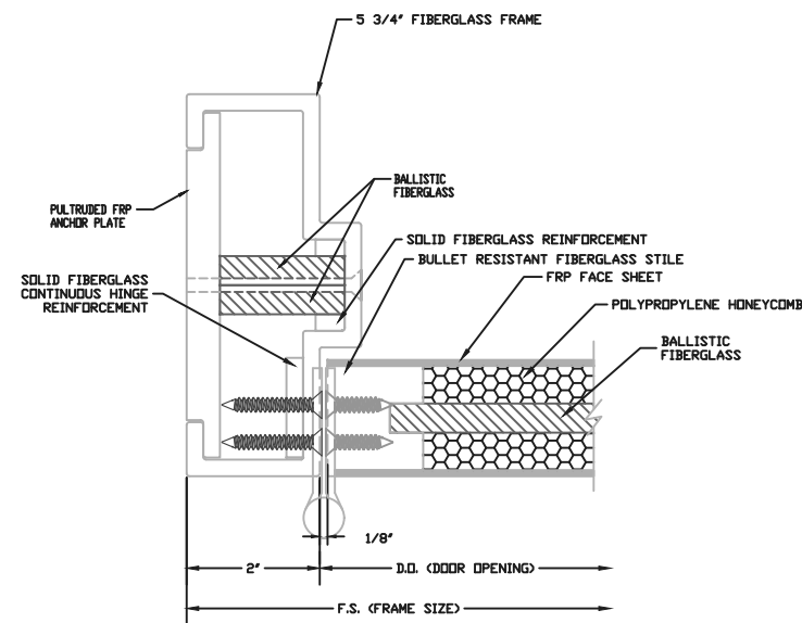
BUTT HINGE JAMB DETAIL
