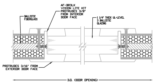
VISION-LITE DETAIL
