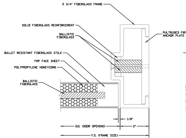
LOCK JAMB DETAIL
