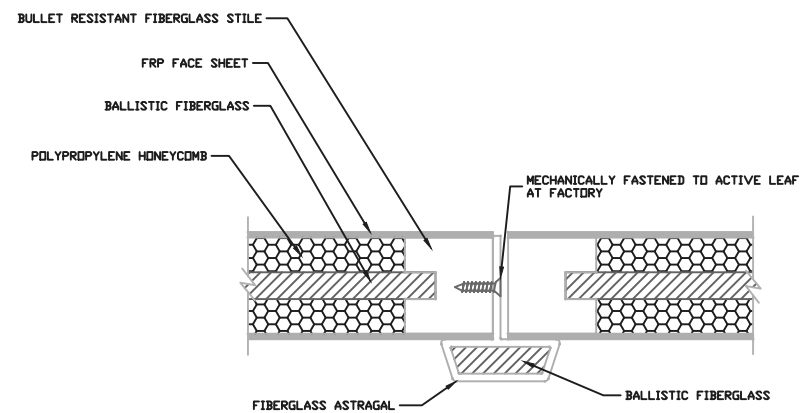
MEETING STILES WITH ASTRAGAL
