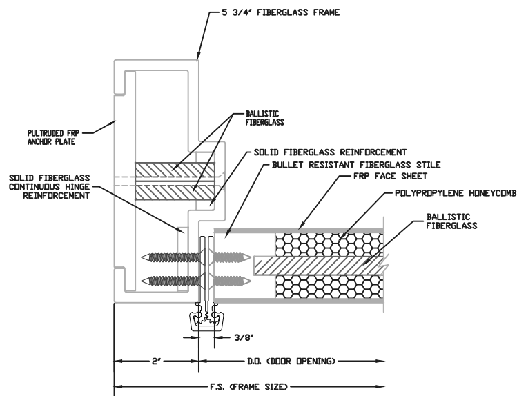
CONTINUOUS HINGE JAMB DETAIL
