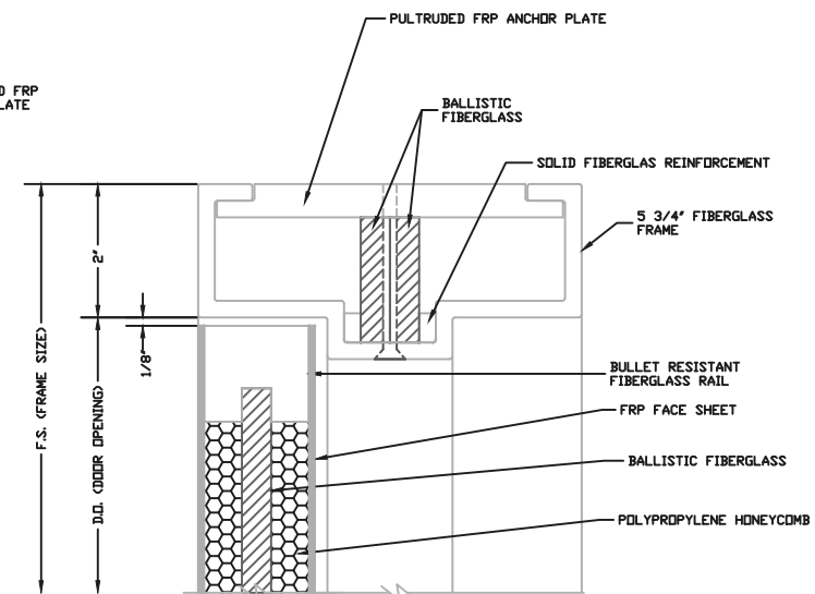
HEAD DETAIL
