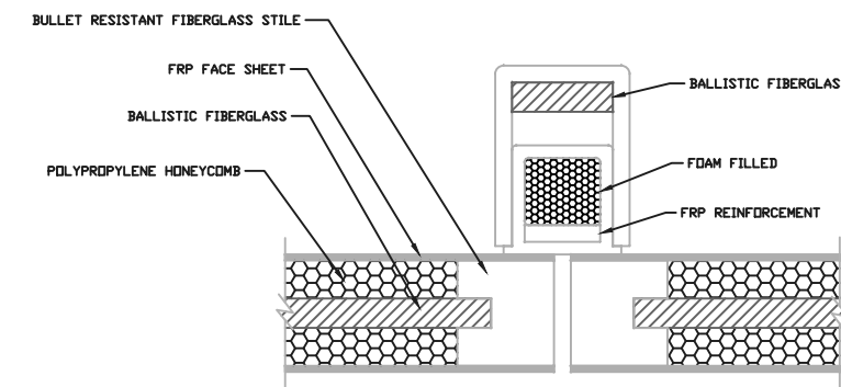
HEAD DETAIL
