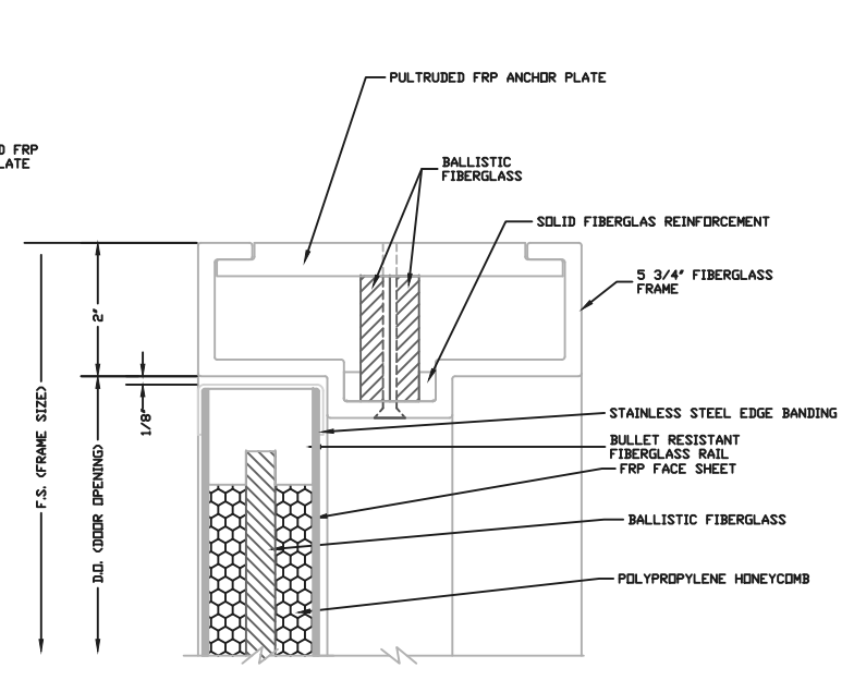
HEAD DETAIL
