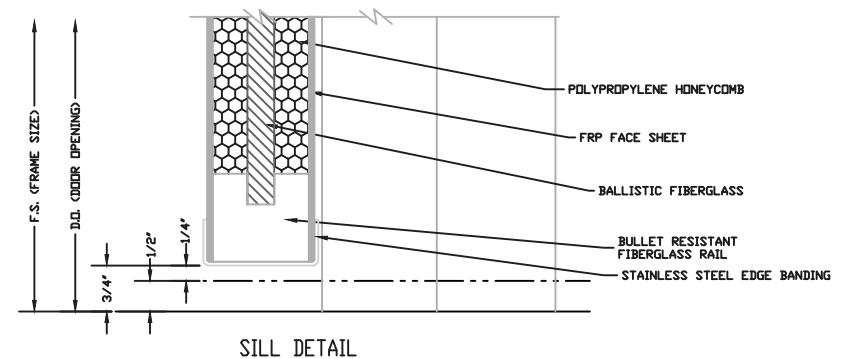
SILL DETAIL
