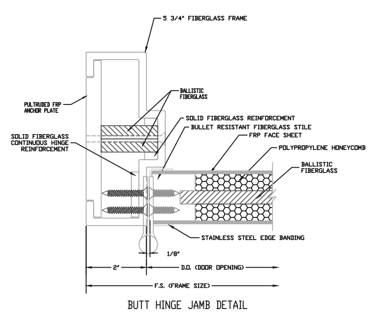
BUTT HINGE JAMB DETAIL
