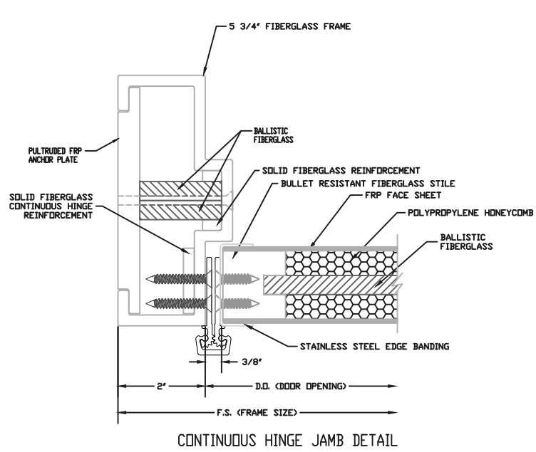
CONTINUOUS HINGE JAMB DETAIL
