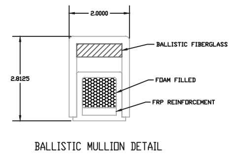
BALLISTIC MULLION DETAIL
