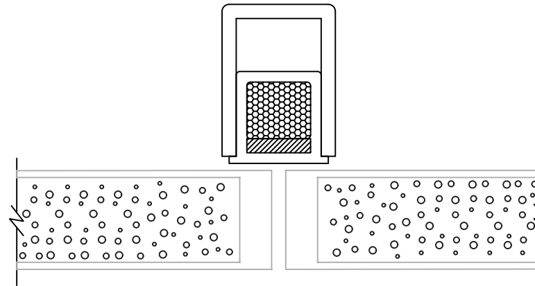
AF REMOVABLE MULLION SHOWN WITH AF-100 DOORS
