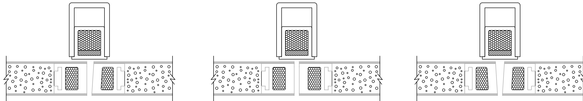
AF REMOVABLE MULLION SHOWN WITH AF COMPOSITE SERIES DOORS
