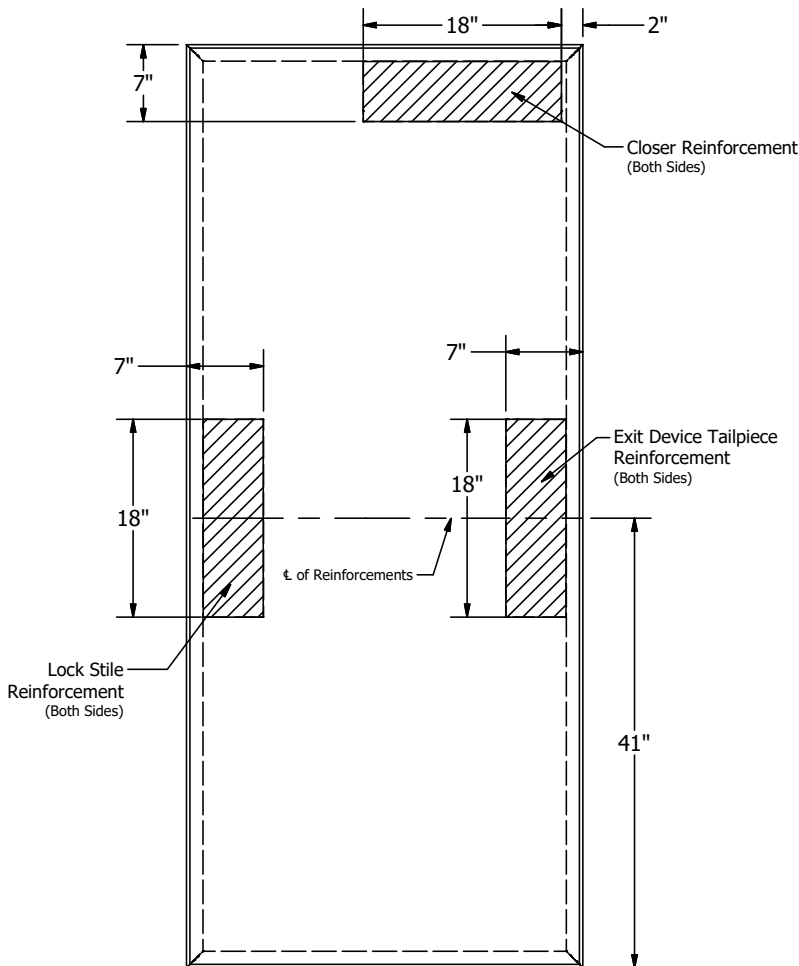
Reinforcement Locations
