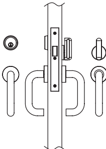
9550 Office - ADA Thumbturn and Single Cylinder
