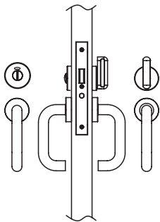
9640 Privacy - ADA Thumbturn, Coin Turn Release with Privacy Indicator
