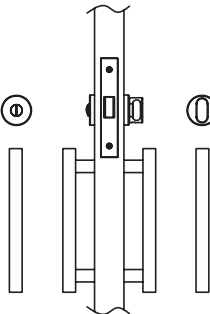
5340 Privacy - ADA Thumbturn, Coin Turn Release
