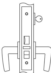
1756 - Entrance or Office, Narrow Stile Mortise Lock with Lever
