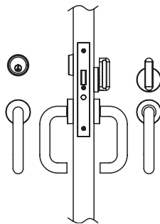
9650 Office - ADA Thumbturn, Single Cylinder
