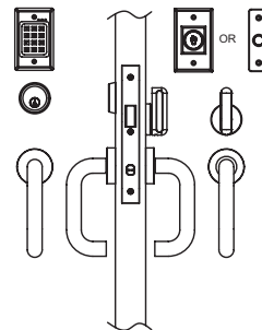
97PT50 Office/Entry - ADA Thumbturn, Single Cylinder
