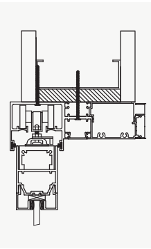
Flush-Mounted Sliding Door System
