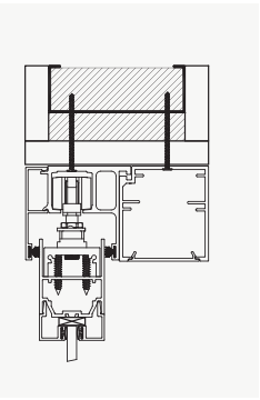
Demountable Wall Sliding Door System
