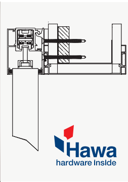
Surface-Mounted Sliding Door System
