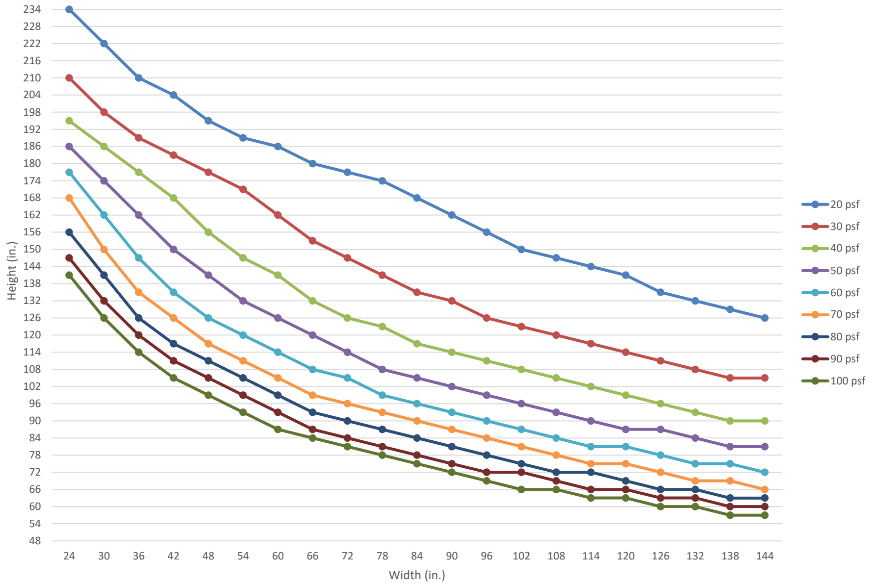
SL-280, 2" x 8" Heavy Duty Framing with Applied Stop
