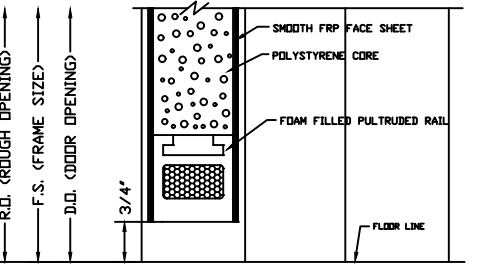
SILL DETAIL (FLUSH BOTTOM)
