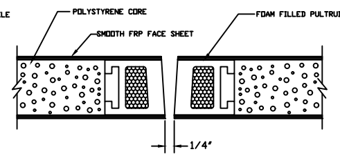
LOCK JAMB DETAIL (OPTIONAL SQUARE STILE)
