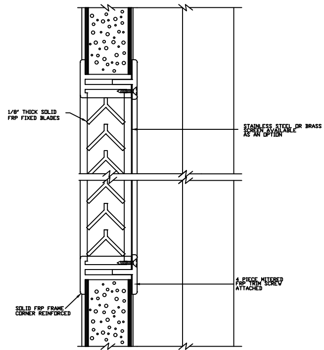
LOUVER WITH INSECT SCREEN DETAIL
