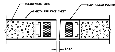
BUTT HINGE JAMB DETAIL (NOT AVAILABLE ON BEVELED STILE)
