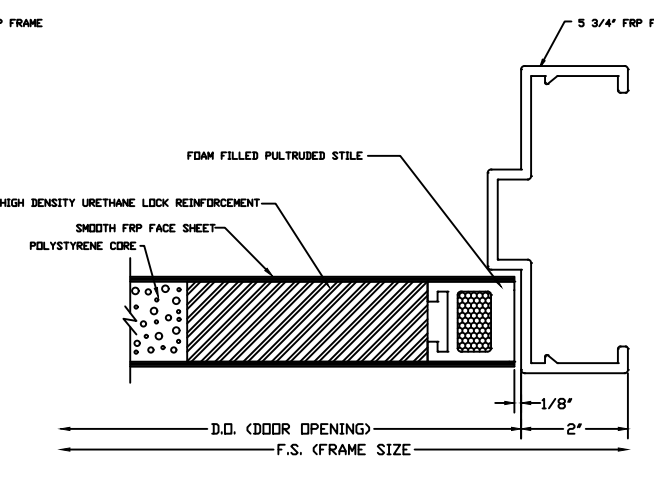
LOCK JAMB DETAIL (OPTIONAL SQUARE STILE)
