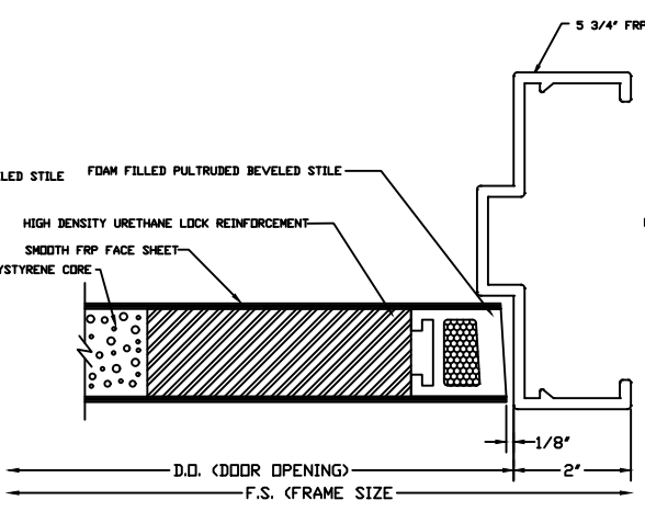
LOCK JAMB DETAIL
