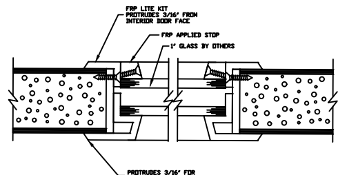
1" GLASS VISION LITE KIT DETAIL
