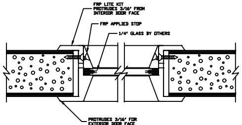
1/4" GLASS VISION LITE KIT DETAIL
