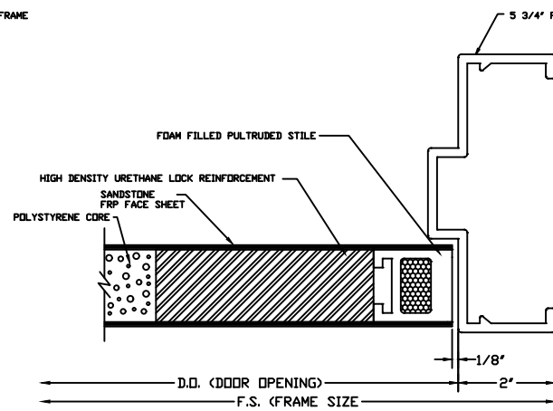
LOCK JAMB DETAIL (OPTIONAL SQUARE STILE)
