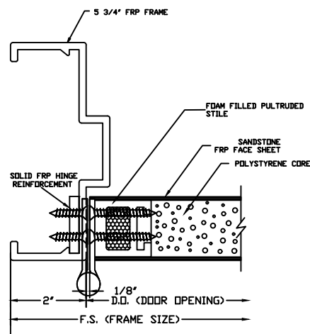
BUTT HINGE JAMB DETAIL (NOT AVAILABLE ON BEVELED STILE)
