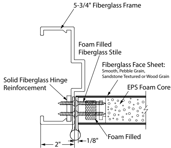
Butt Hinge with Square Hinge Stile (not available on beveled stile)
