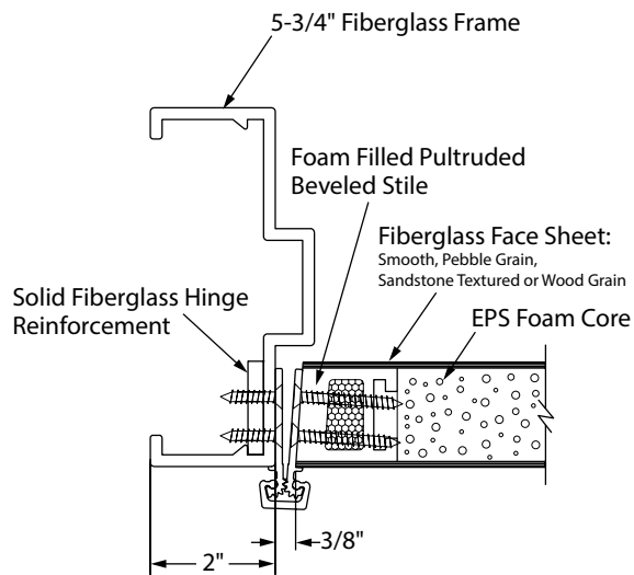
Continuous Hinge with Beveled Hinge Stile
