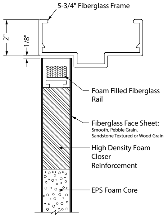
Top Rail
